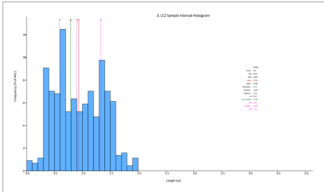
Figure 14.9 Drilling Sample Lengths in the JL LCZ
