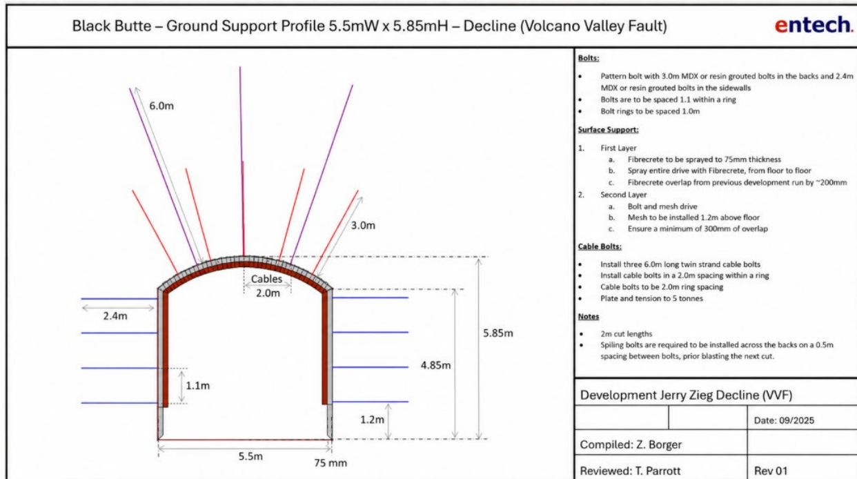
Figure 16.18 13 Ground support layout for Jerry Zieg Decline development – VVF (Entech, 2026)
