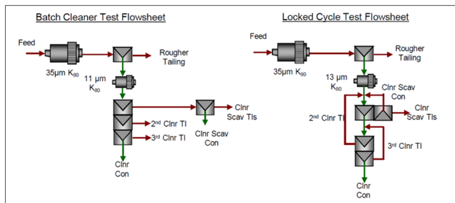
Figure 13.10 JL UCZ- JL LCZ Flotation Flowsheet Development
