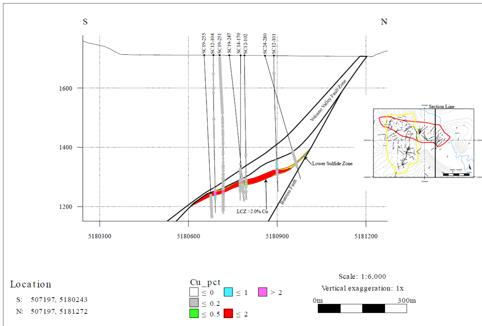
Figure 10.5 Cross section of the Johnny Lee LCZ; view to west. See inset for line of section
