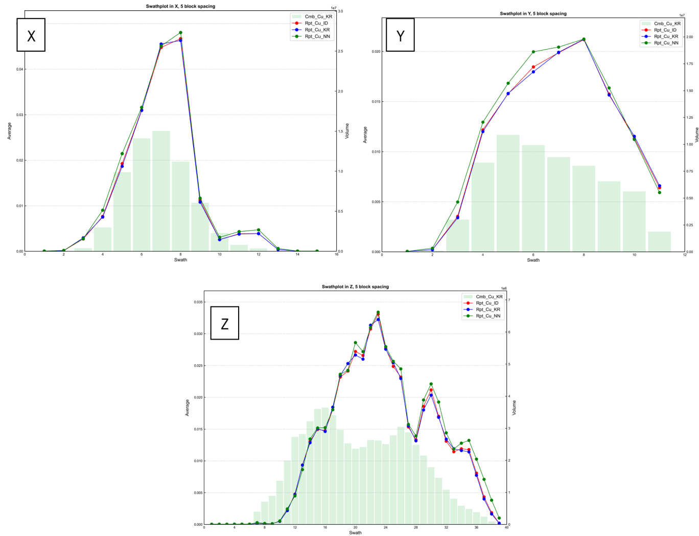
Figure 14.26 Lowry Swath Plots
