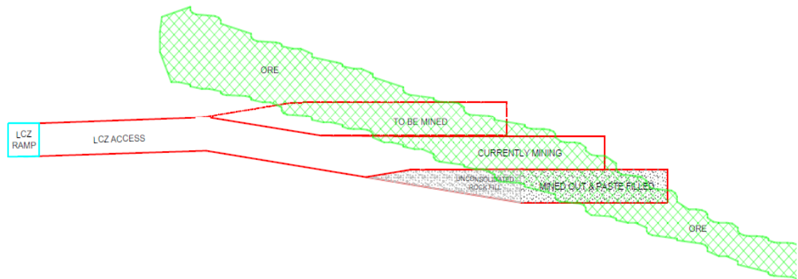
Figure 16.27 Section View Schematic JL LCZ Mining Method (SRA, 2022)
