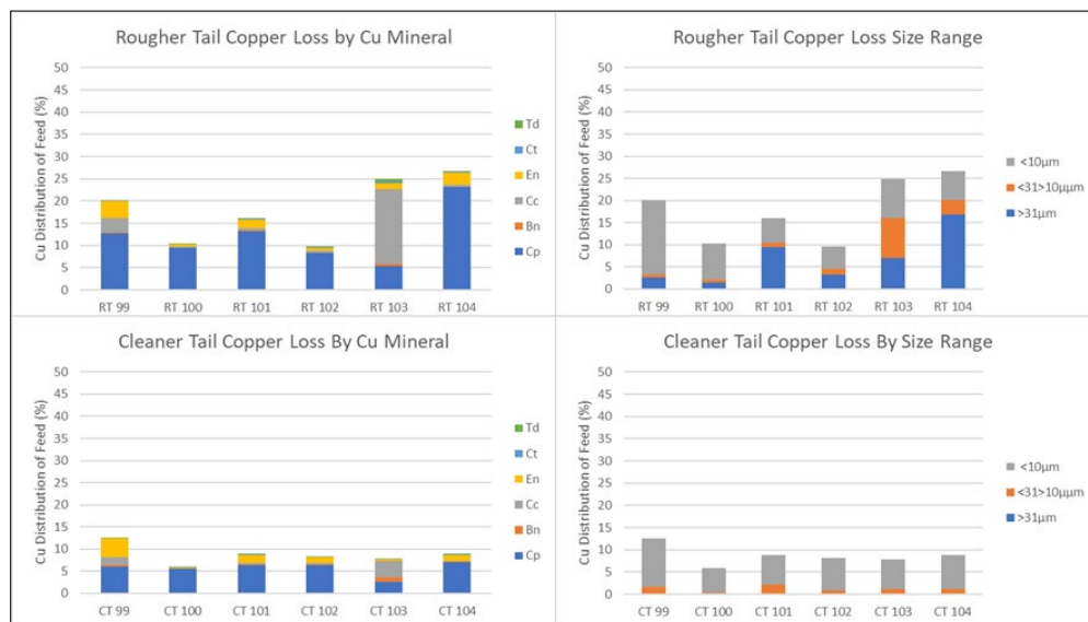
Figure 13.9 QEMSCAN – Mineral Identification – Rougher and Cleaner Tails
