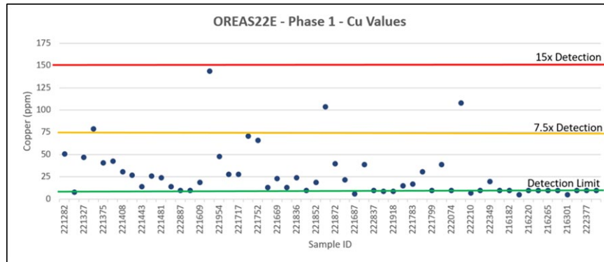
Figure 11.27 Cu results of pulp blank OREAS-22e during the 2018 Phase 1 drill program
