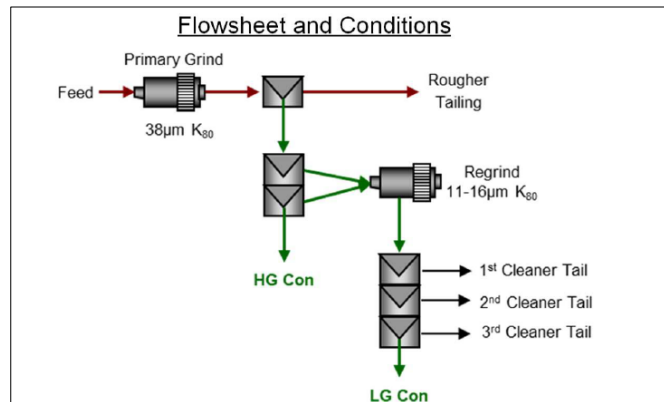
Figure 13.25 Cleaner Test Flowsheet
