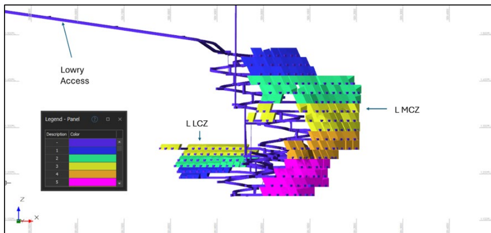
Figure 16.28 View Looking North of LMCZ and LLCZ Mining Panels (SRA, 2022)
