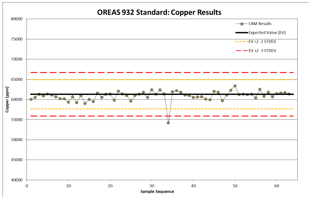
Figure 11.24 OREAS-932 Cu values from the 2023–2025 drill program
