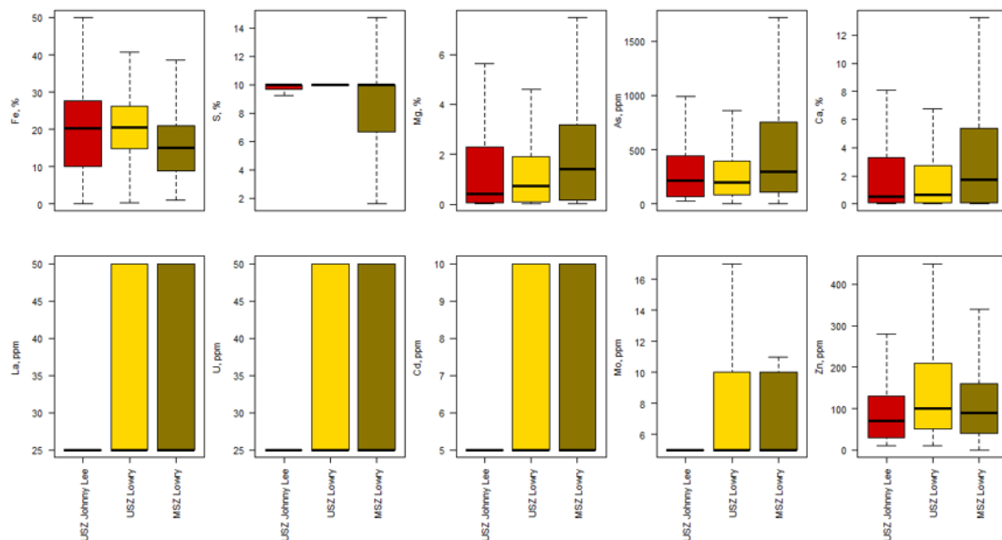
Figure 20.12 Boxplots of select parameters from multi-element testing of the Sulfide Zone waste rock in the Johnny Lee (JL) and Lowry (L) deposits. (RESPEC, 2026)
