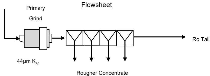
Figure 13.16 Rougher Kinetic Test Flowsheet
