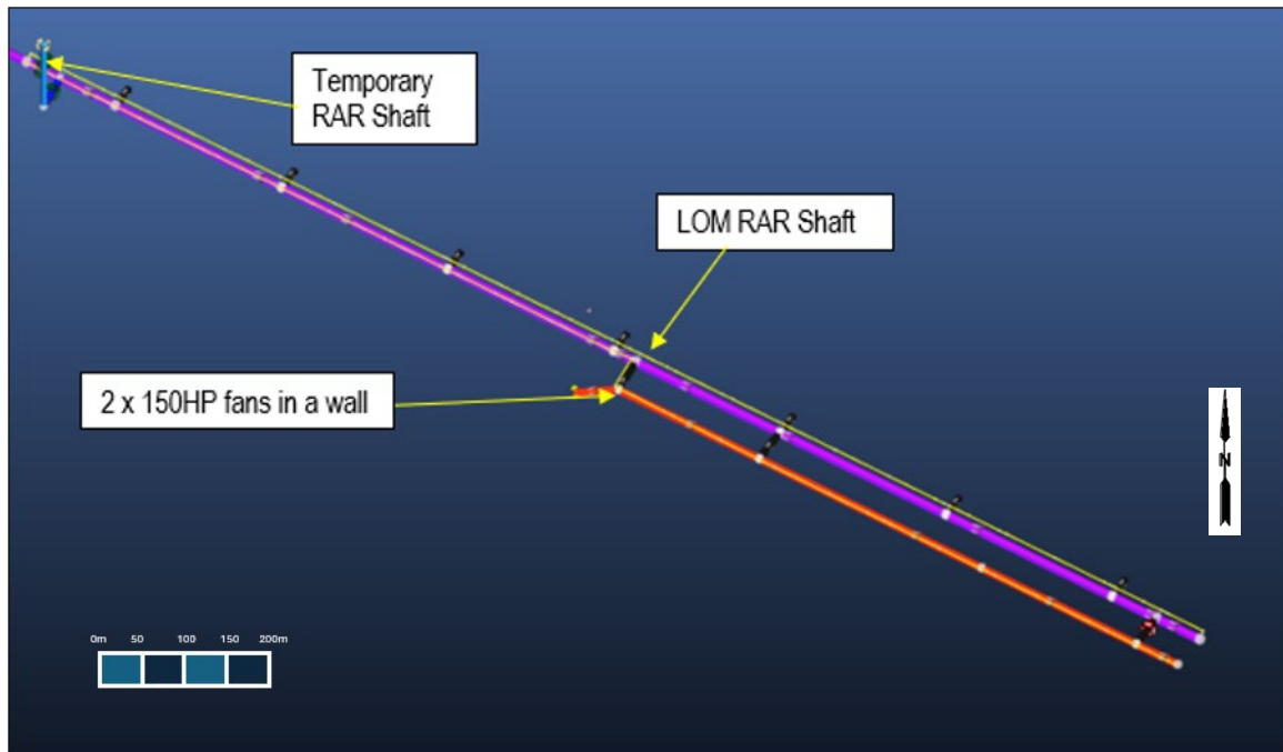
Figure 16.34 Plan View of Lowry Initial Decline Ventilation Layout (Entech, 2026)
