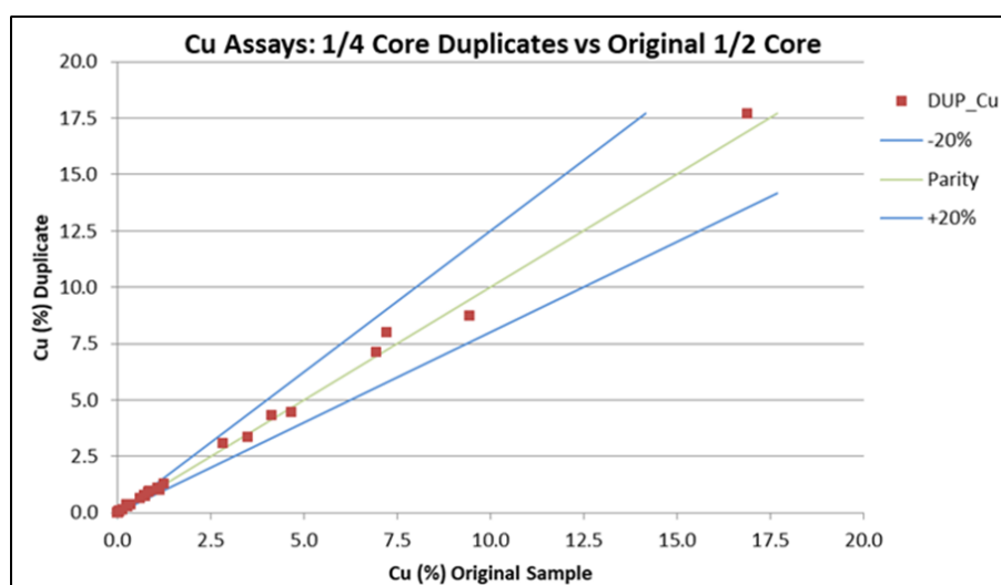
Figure 11.33 Comparison of Cu analyses from original and field duplicates from the 2014 drill program
