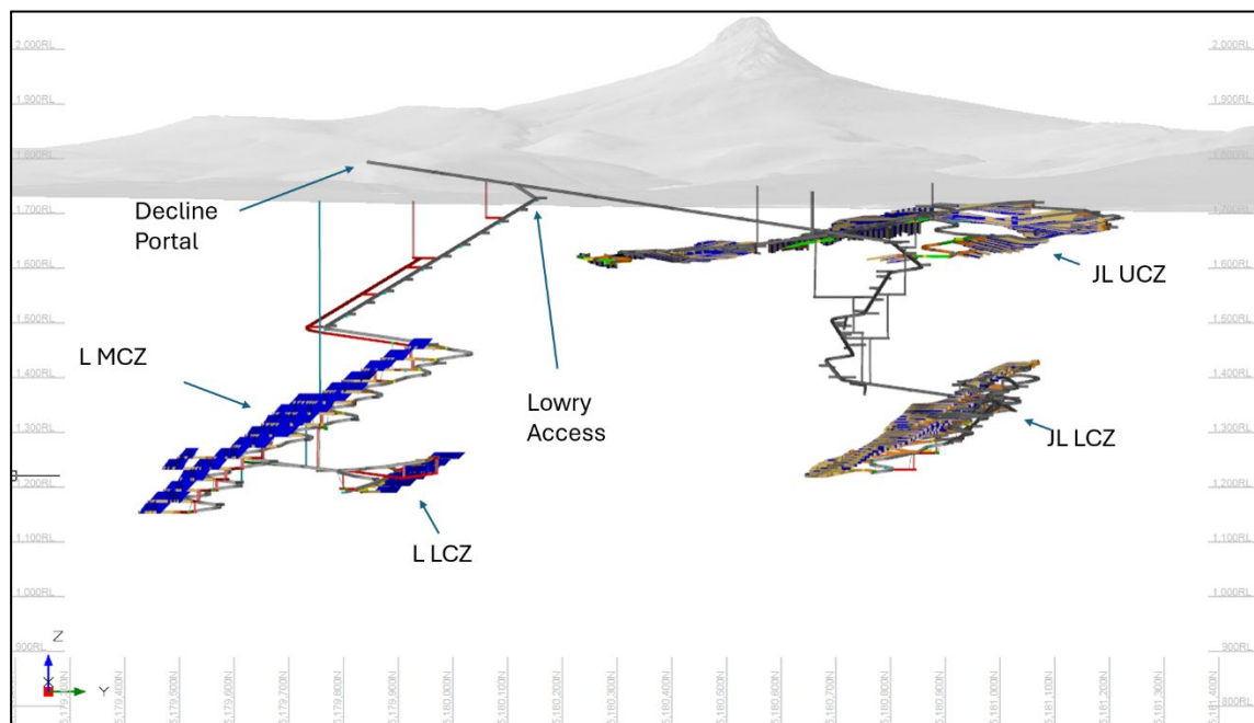
Figure 16.30 View of UG Design from the East (Entech, 2026)
