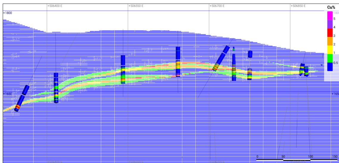
Figure 14.16 JL UCZ Section N5180805 ( \pm 17.5 m) Looking North at Cu Block Model versus Cu Composites
