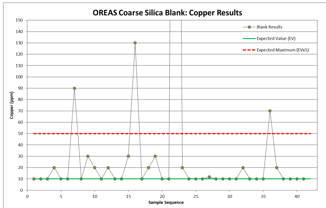
Figure 11.31 Cu results for coarse blanks for the 2023–2025 drill program
