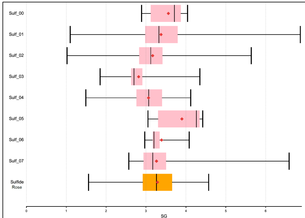
Figure 14.15 Box and Whisker Plot of SG by Sulfide Domain in the Lowry deposit
