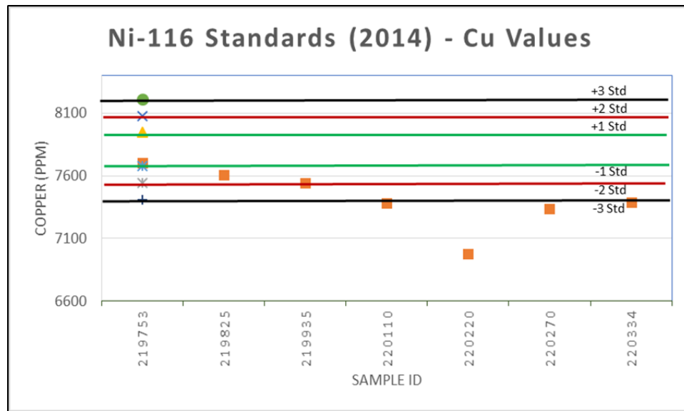
Figure 11.5 Ni-116 Cu values from the 2014 drill program
