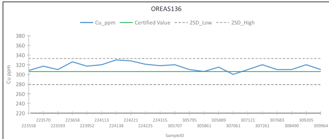
Figure 11.16 OREAS-136 Cu values from the 2021/22 drill program
