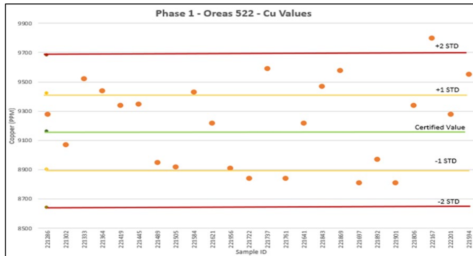
Figure 11.8 ORES-522 Cu values from the 2018 Phase 1 drill program
