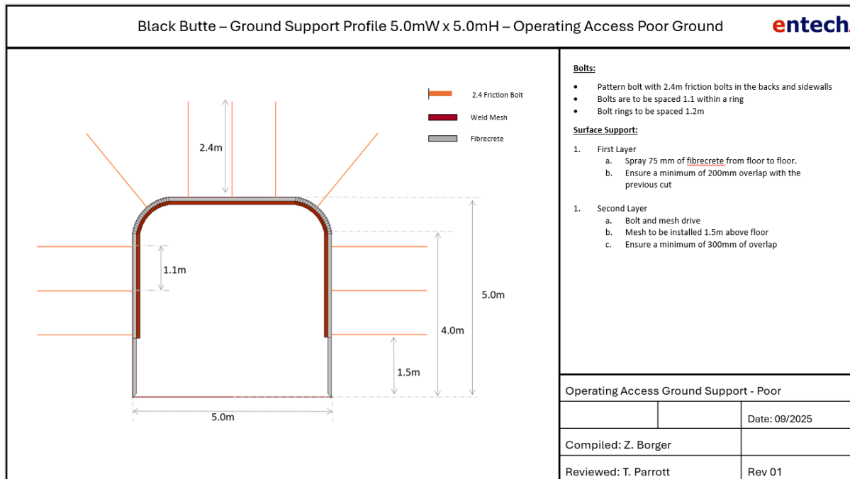
Figure 16.24 17 Ground support layout for Access development - Poor Ground (Entech, 2026)
