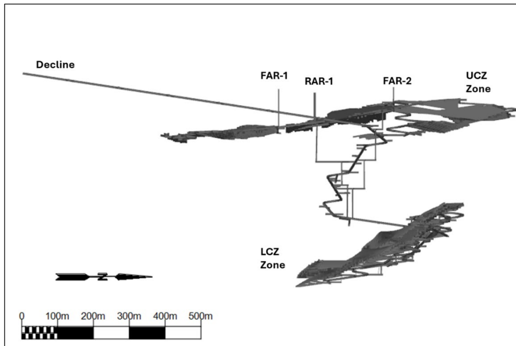
Figure 1.2 View of JL UG Design from the East (Entech 2025)
