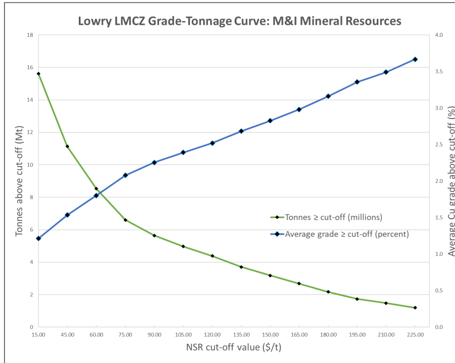
Figure 14.33 Grade-Tonnage Curve for the Lowry LMCZ Measured & Indicated Mineral Resources
