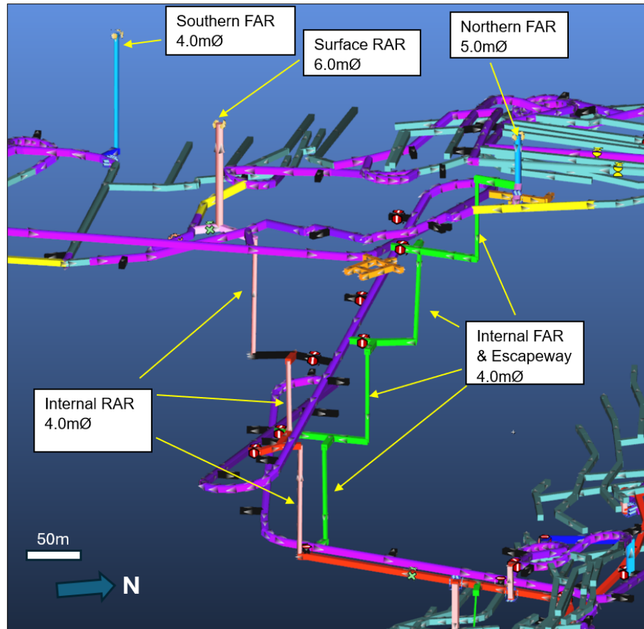
Figure 16.33 Isometric view from SE of JL LCZ Fresh and Return Air Route (Entech 2025)
