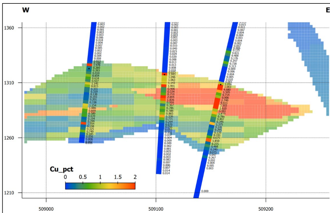
Figure 14.23 Cross-section N5179640 Comparing Cu Composites to Block Grades
