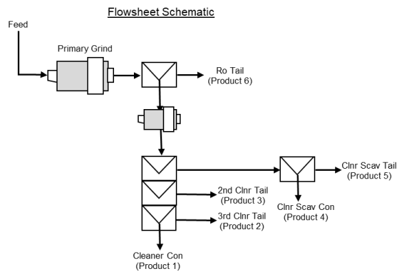
Figure 13.22 Flowsheet and reagent condition setup
