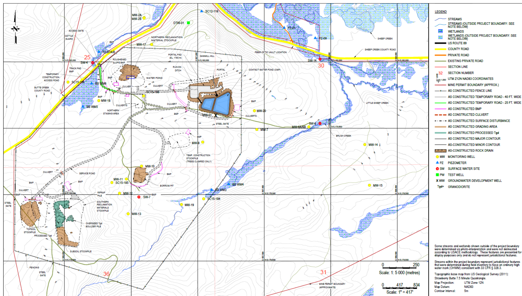
Figure 18.3 As-constructed 2020 Phase 1 Construction
