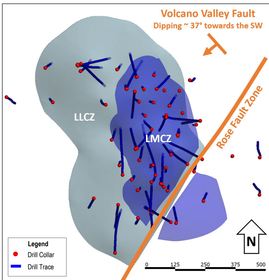
Figure 10.6 Plan view of Lowry MCZ (LMCZ) and Lowry LCZ (LLCZ)
