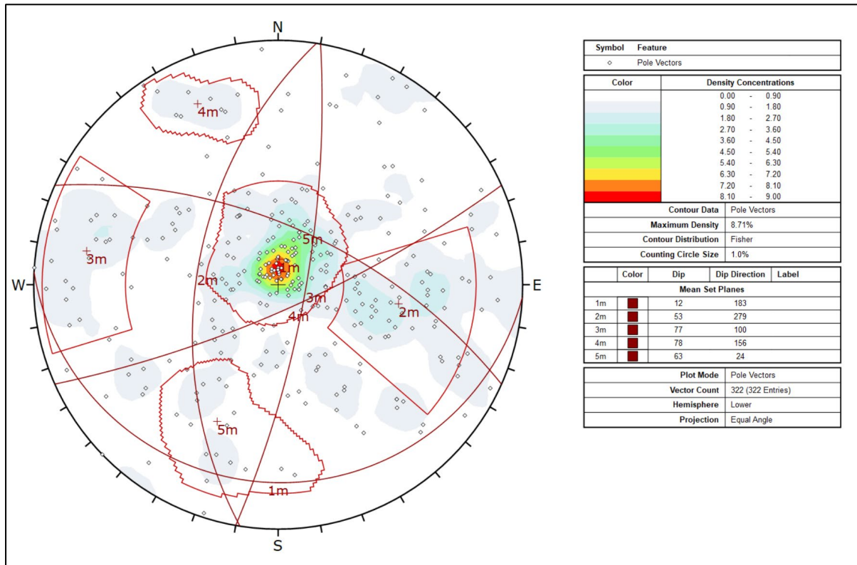
Figure 16.12 8Stereonet plot displaying orientated structure for the UCZ at Johnny Lee (Entech, 2026)
