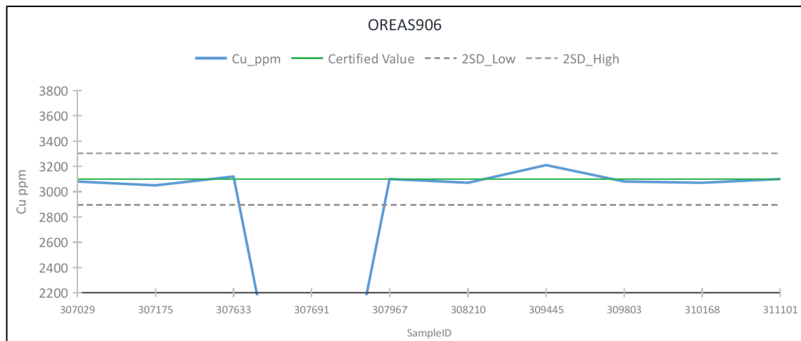
Figure 11.18 OREAS-906 Cu values from the 2021/22 drill program
