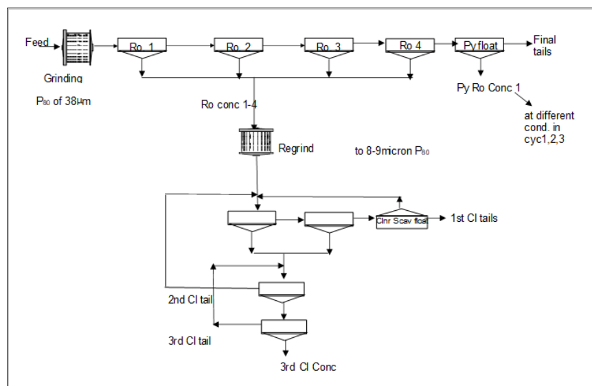
Figure 13.3 LCT PEA Flowsheet
