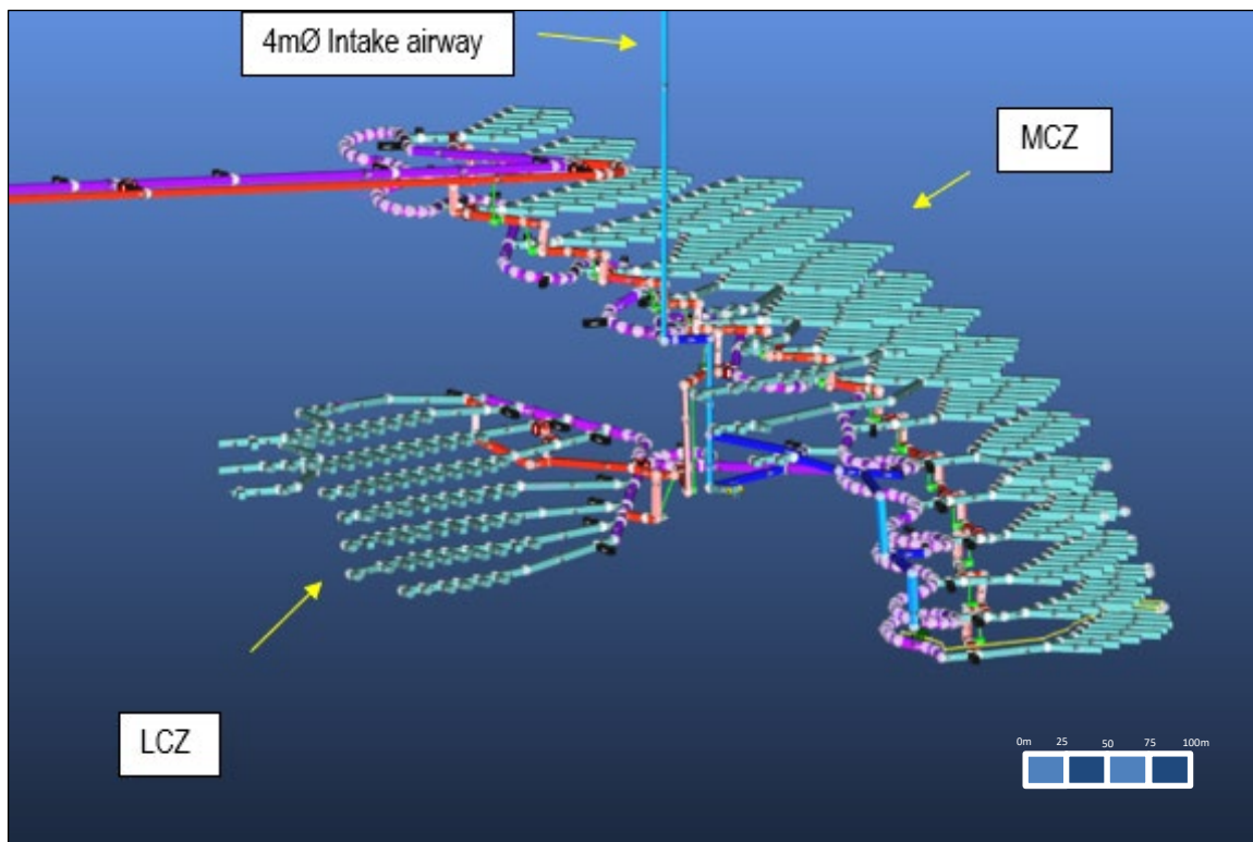
Figure 16.36 Isometric View from West of Final Lowry Primary Ventilation Layout (Entech, 2026)
