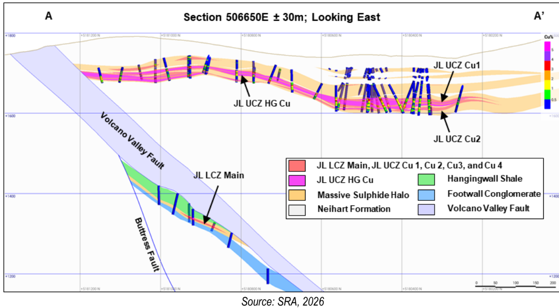
Figure 14.2 Cross-section of the JL UCZ Halo and Vein models
