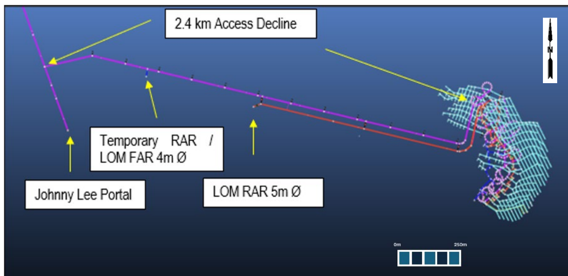
Figure 16.35 Plan view of Lowry Decline & Primary Ventilation Layout (Entech, 2026)
