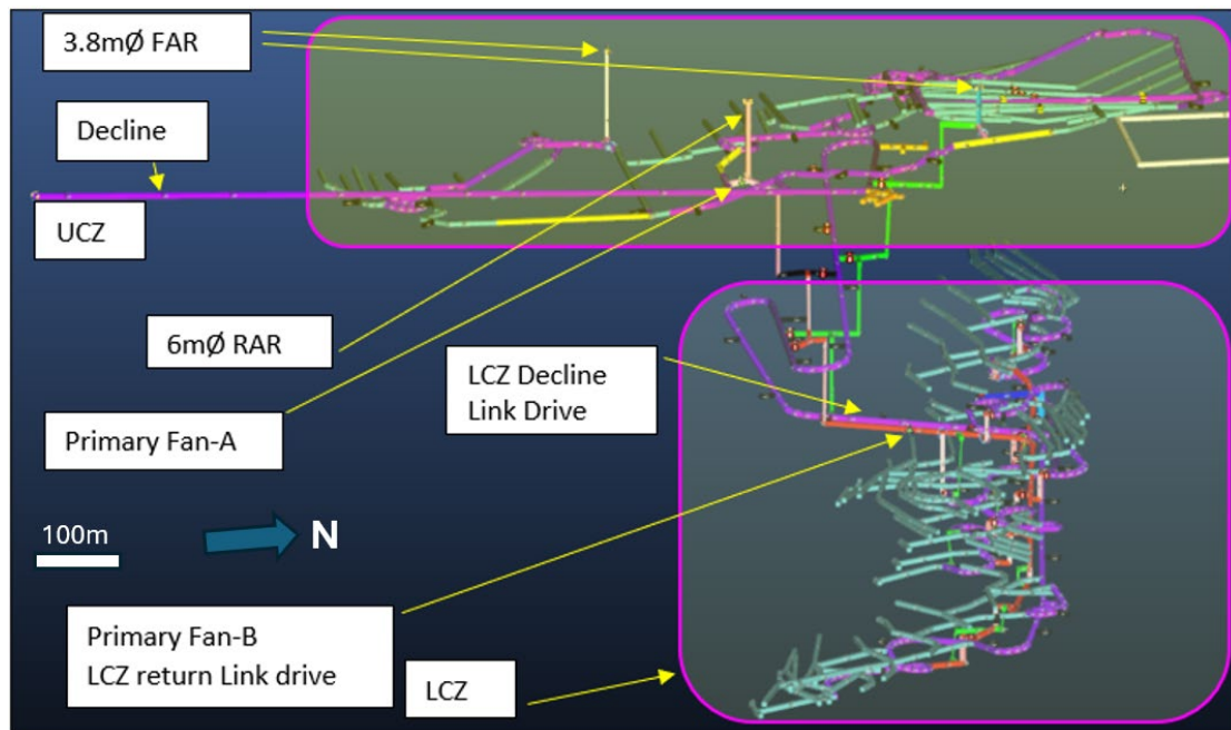
Figure 16.32 Isometric View from SE of Primary Ventilation Plan Schematic (Entech 2025)
