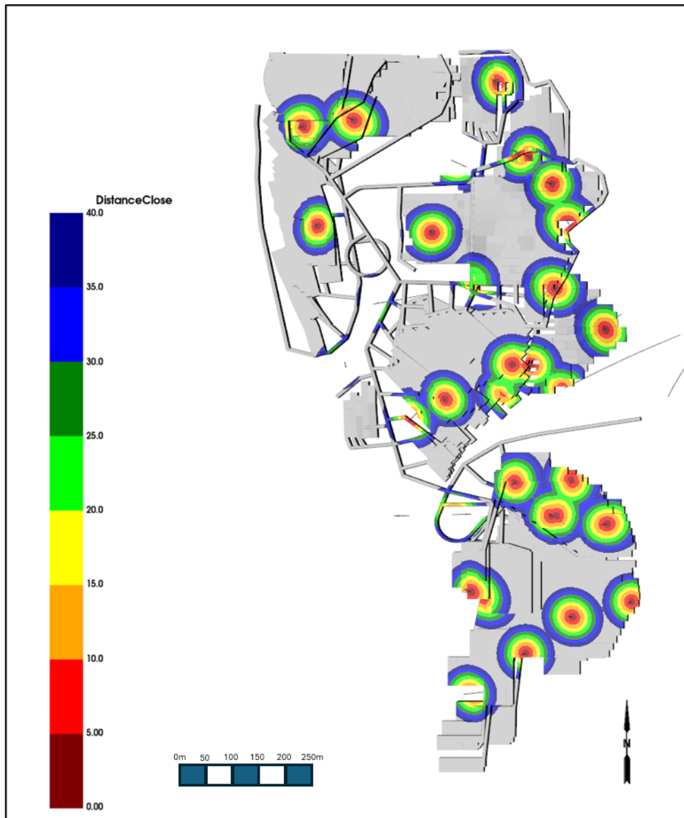
Figure 16.1 Plan view Geotechnical drill hole coverage for Johnny Lee UCZ with a heat map extrapolated 40 m (Entech, 2025)
