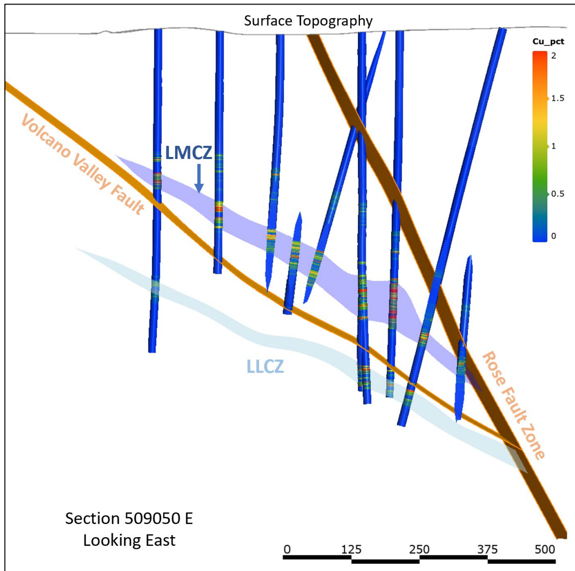
Figure 10.7 Cross-section of the Lowry MCZ (LMCZ) and Lowry LCZ (LLCZ), looking east
