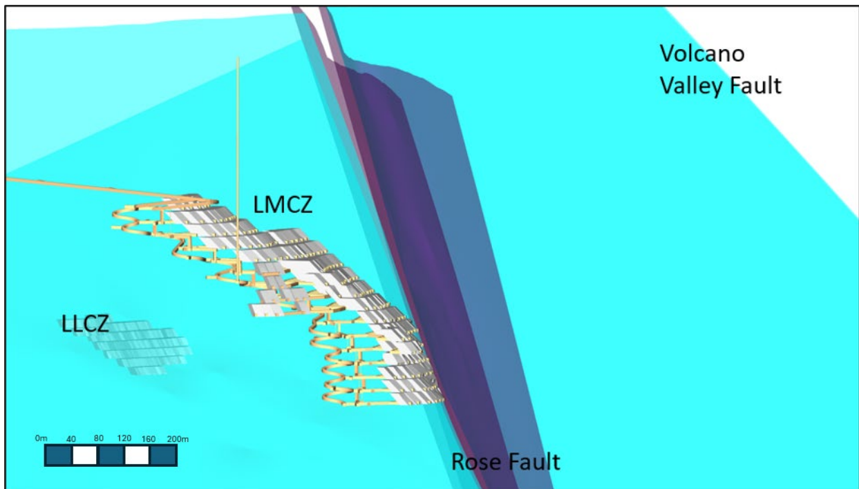
Figure 16.7 Lowry mining zone looking northeast, displaying the major structures (Entech, 2026)
