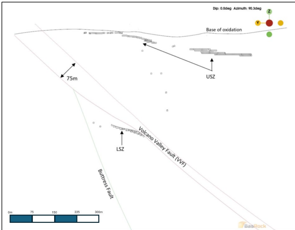
Figure 16.6 Cross-section view looking east, displaying the major structures for Johnny Lee. (Entech, 2025)
