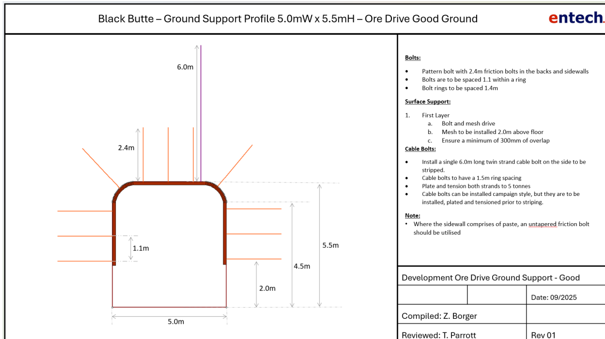
Figure 16.19 14 Ground support layout for ore drive development - good ground (Entech, 2026)
