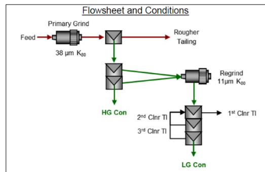
Figure 13.28 LCT Flowsheet
