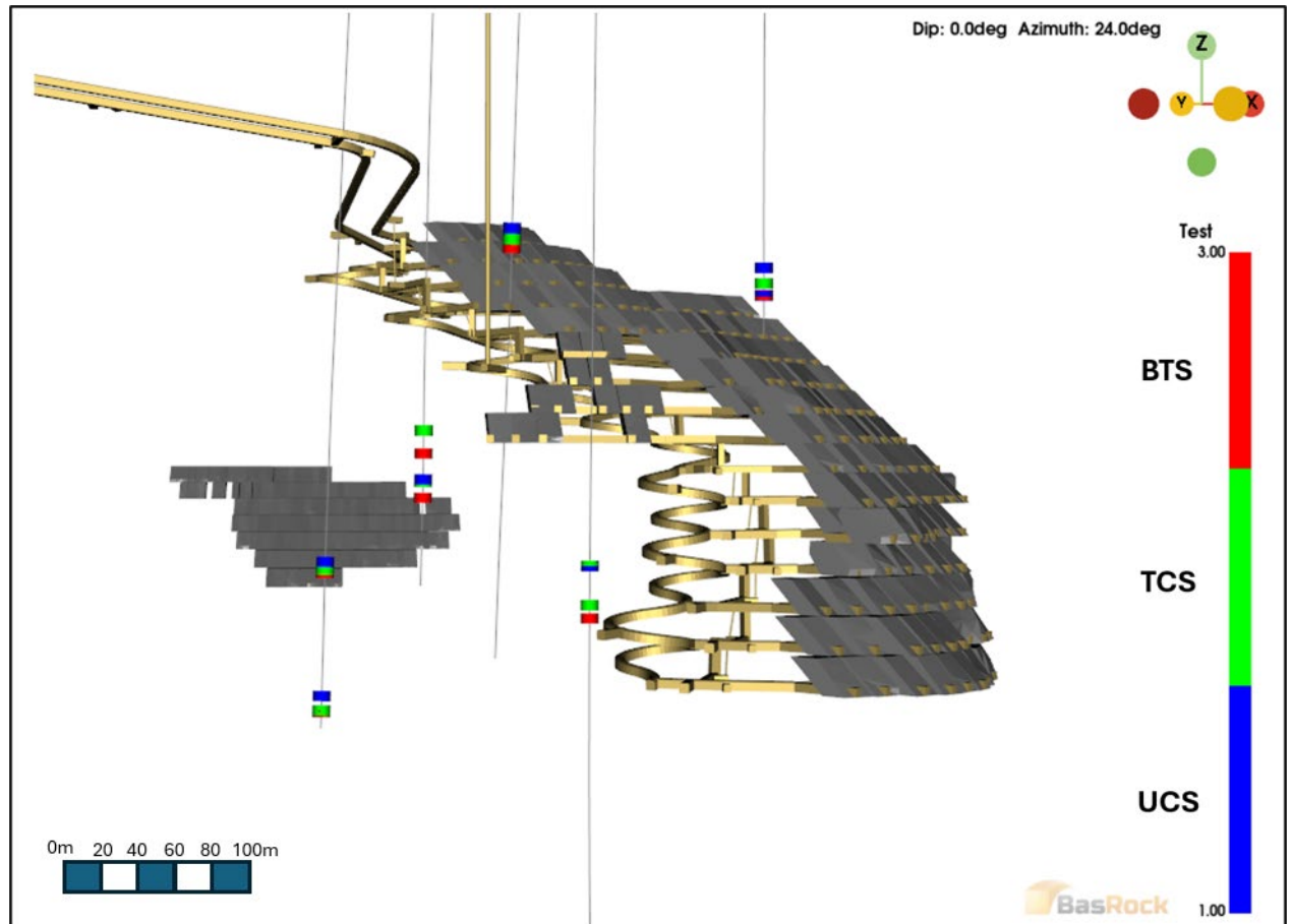
Figure 16.22 View looking north-northeast showing the sample locations for Lowry (Entech, 2026)
