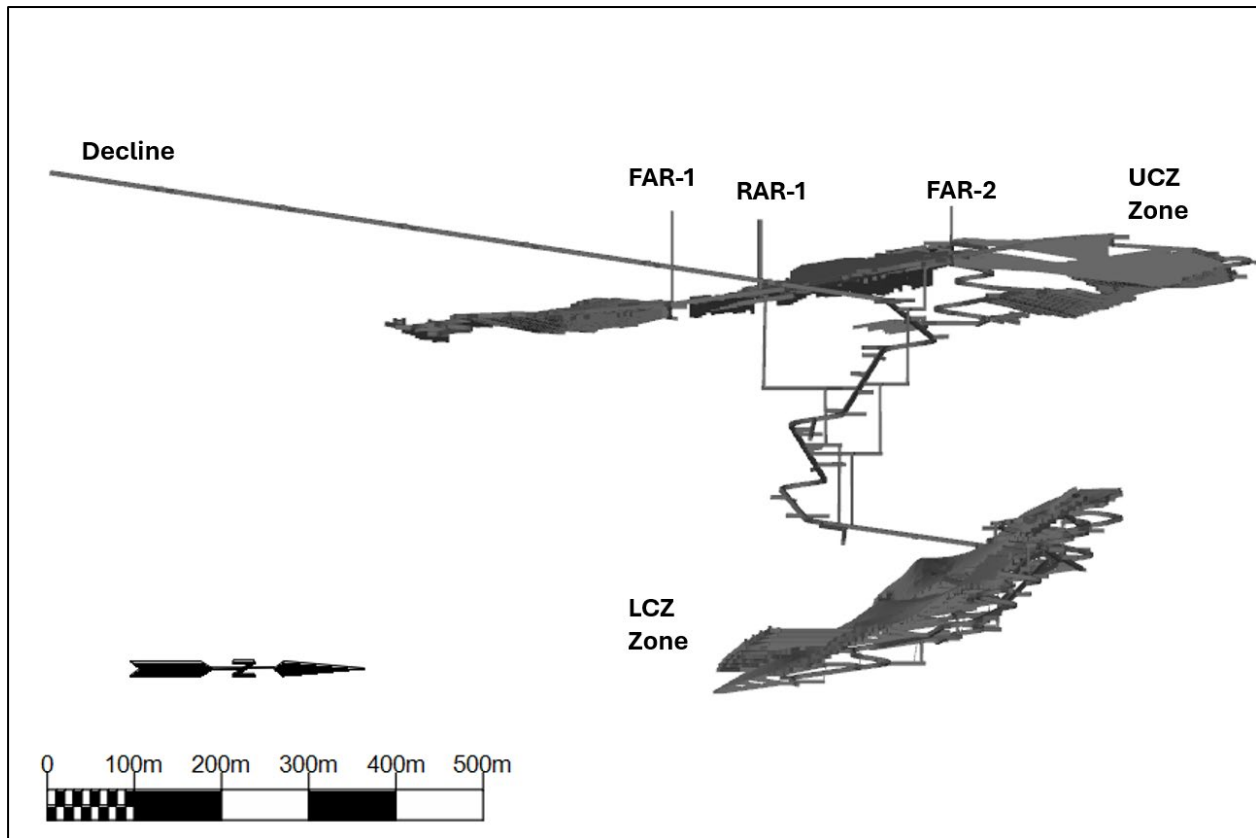
Figure 16.29 Isometric View JL UG Design from the Esst (Entech, 2025)
