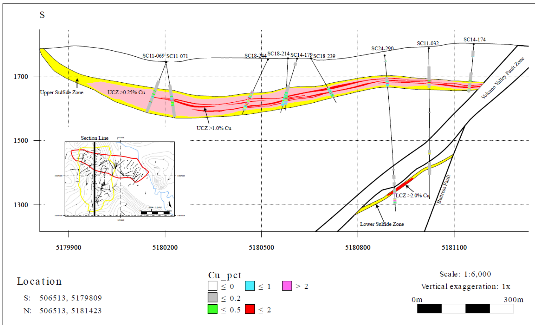
Figure 10.4 Cross-section of the Johnny Lee Deposit; view to west. See inset for line of section
