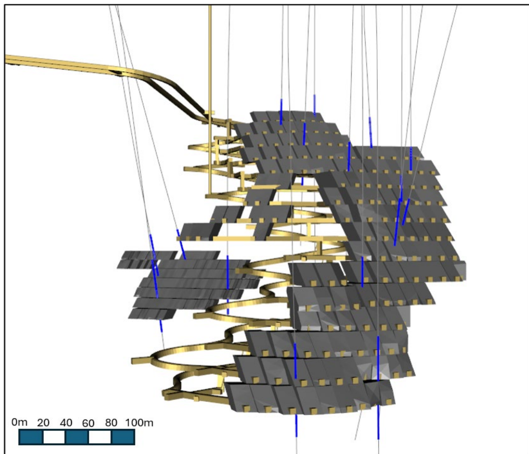
Figure 16.21 15 View looking north of the proposed mine at Lowry showing the distribution of geotechnical drilling data collected. (Colors arbitrary) (Entech, 2026)
