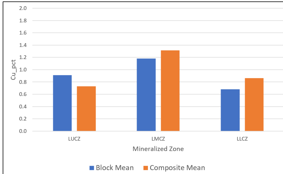
Figure 14.24 Comparison of Lowry Mean Cu Grades by Mineralized Zone for Composites (orange) and Blocks (blue)
