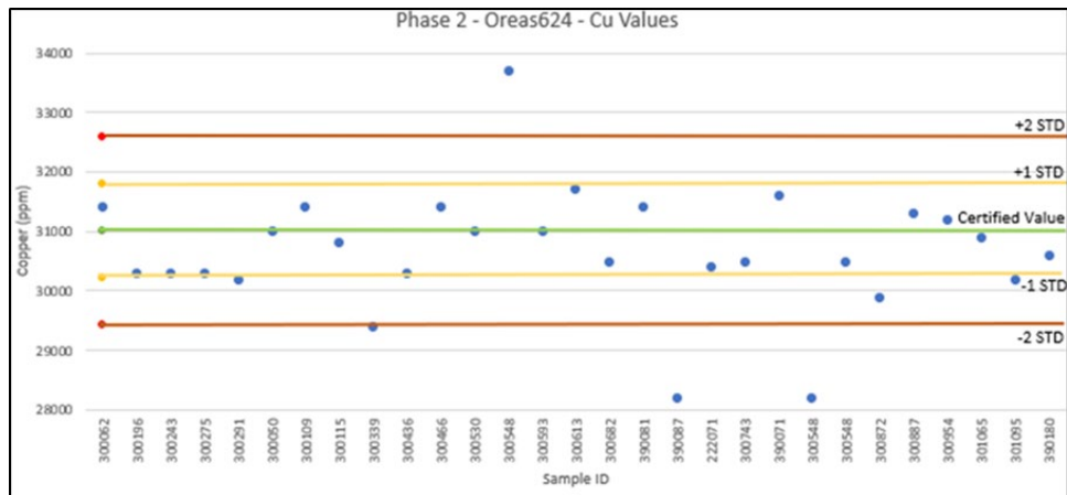
Figure 11.12 OREAS-624 Cu values from the 2018/19 Phase 2 drill program
