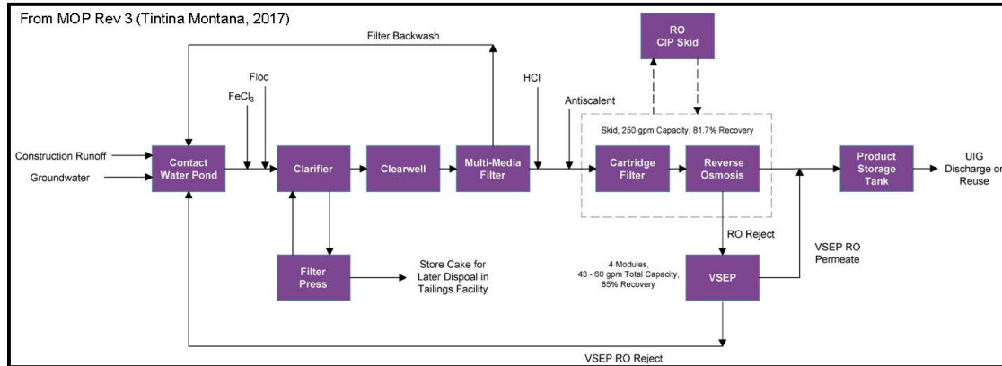
Figure 20.17 Water Treatment Construction Phase Process Flow Diagram
