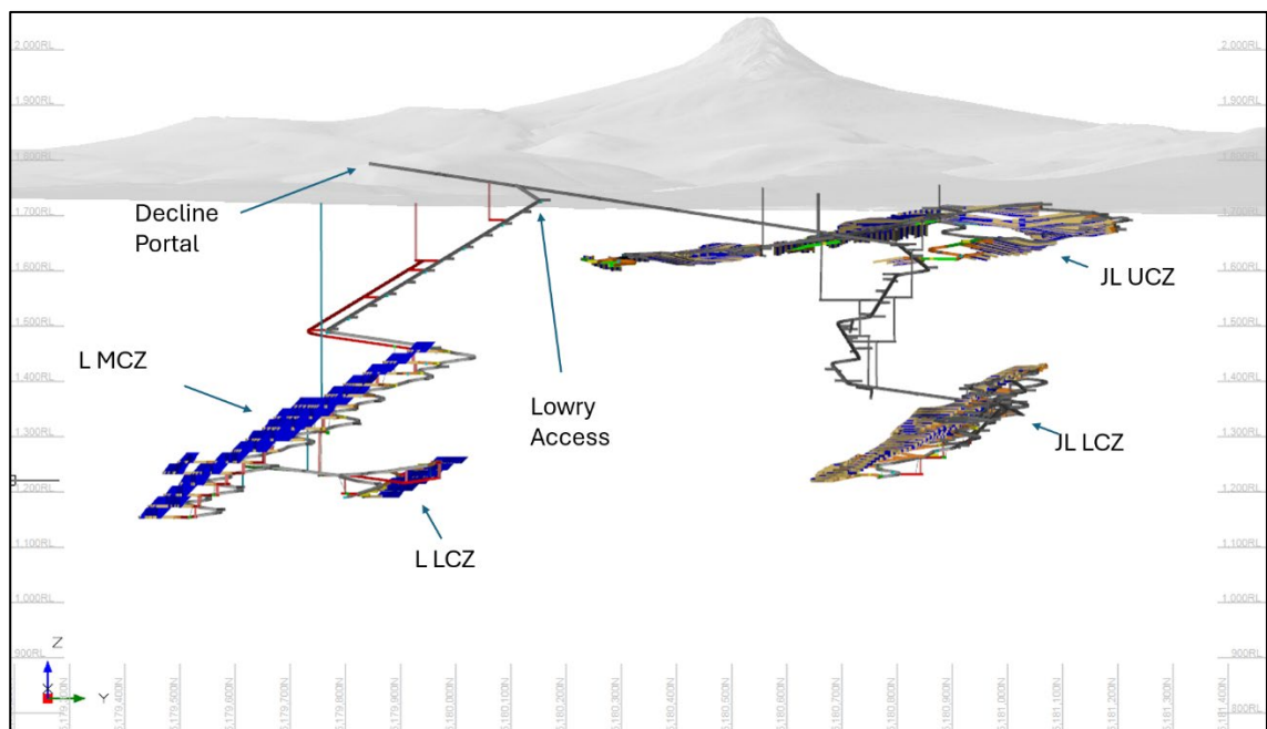
Figure 1.3 View of Lowry and JL UG Design from the East (Entech, 2026)
