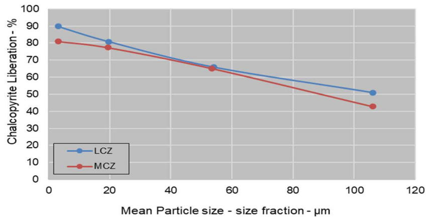
Figure 13.14 Baseline Cu Rougher Performance
