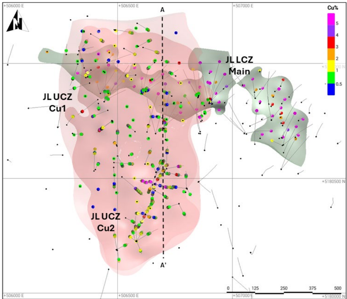
Figure 14.1 Plan view of the JL UCZ and JL LCZ Wireframes and Mineralized Composites
