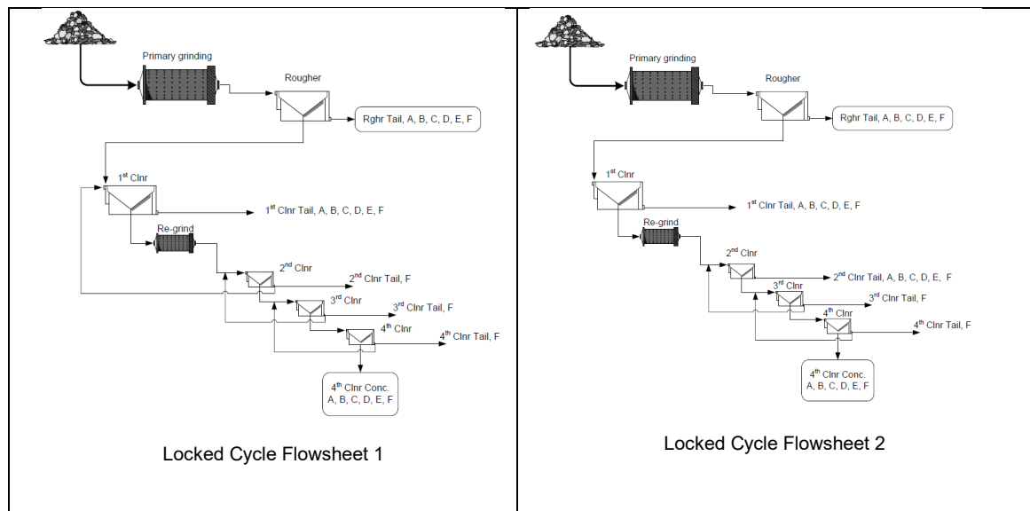
Figure 13.6 JL UCZ Development Composite LCT Flowsheets
