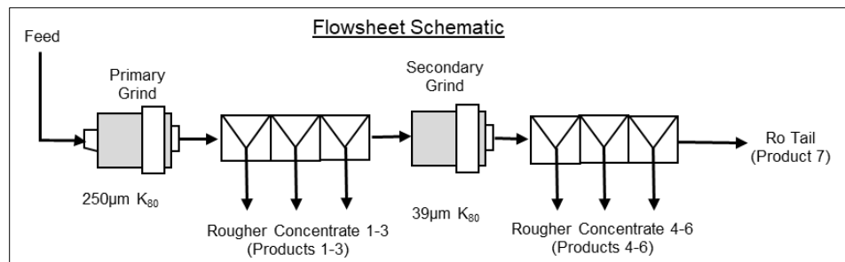
Figure 13.19 MF2 Flowsheet Option
