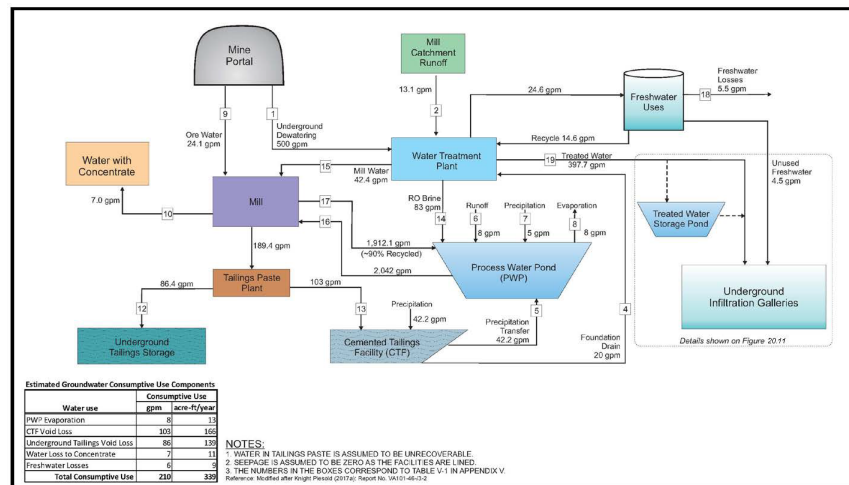
Figure 20.15 Average Annualized Water Balance During Mining Operations – Johnny Lee
