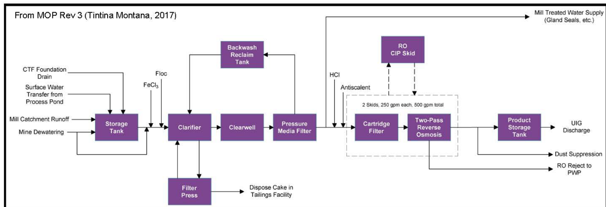
Figure 20.18 Water Treatment Operational Phase Process Flow Diagram
