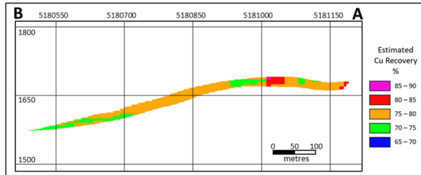
Figure 13.32 Cross-section A to B
