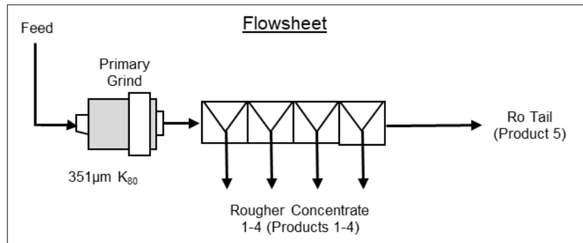
Figure 13.21 Flash Rougher Flowsheet
