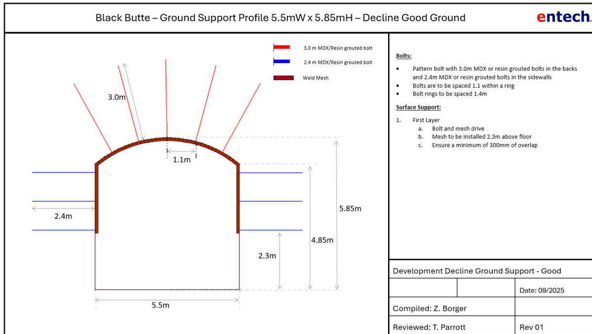
Figure 16.23 16 Ground support layout for Decline development - Good Ground (Entech, 2026)
