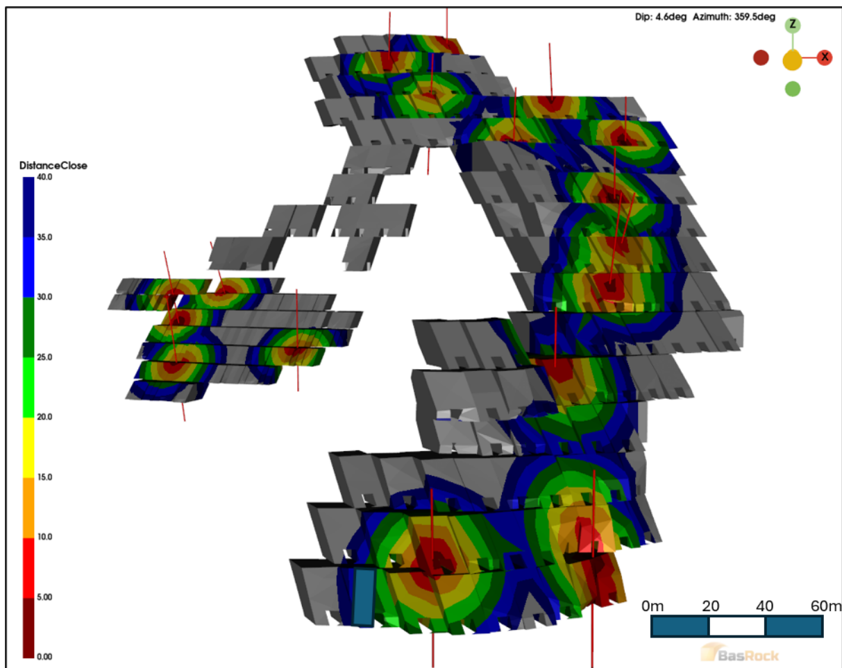
Figure 16.3 1Looking North Geotechnical drill hole coverage for Lowry with a heat map extrapolated 40 m (Entech, 2026)
