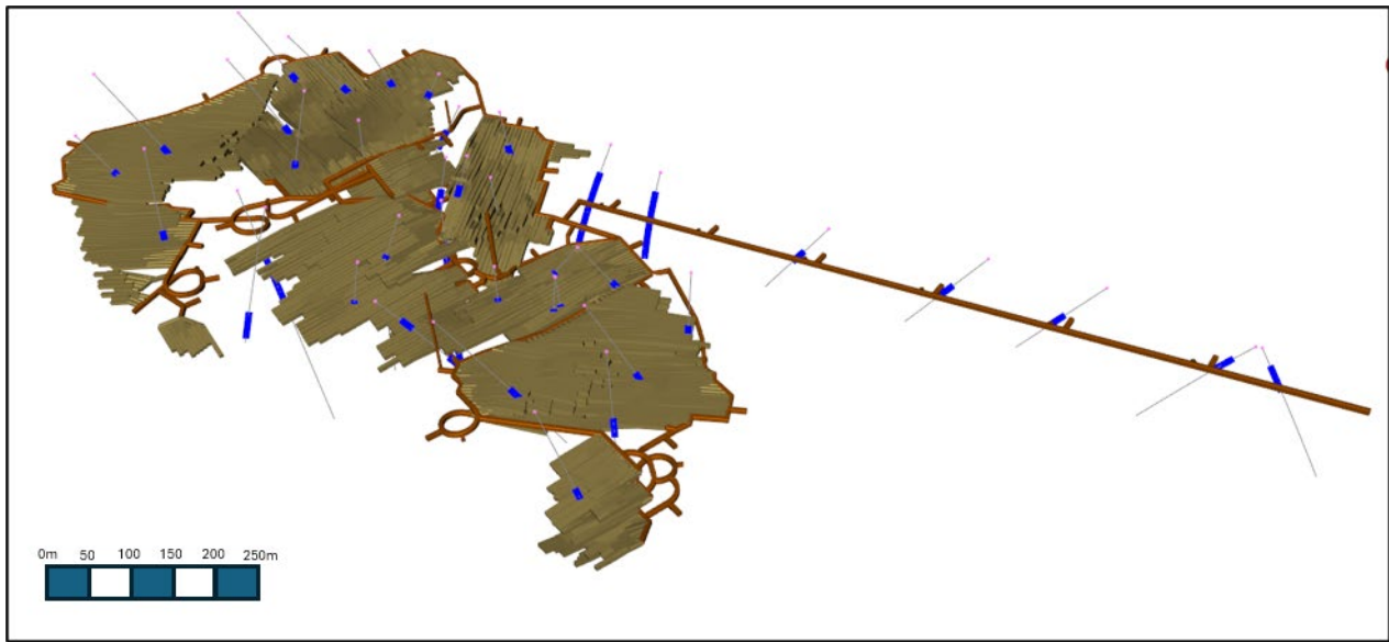
Figure 16.8 4 Oblique plan view of the proposed UCZ and initial JZ decline development at Johnny Lee, showing the distribution of geotechnical drilling data collected (Entech, 2025)
