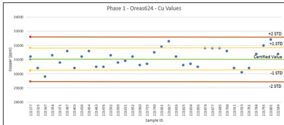
Figure 11.7 ORES-624 Cu values from the 2018 Phase 1 drill program
