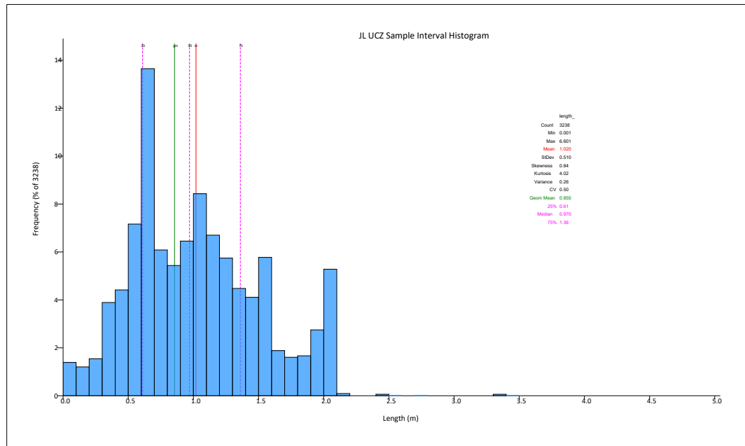
Figure 14.8 Drilling Sample Lengths in the JL UCZ
