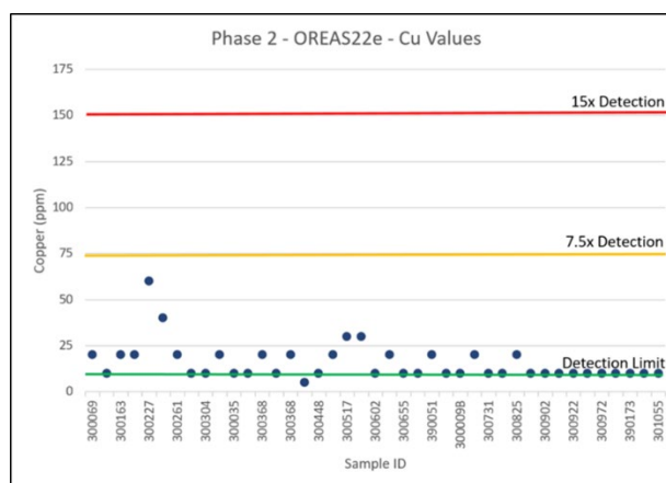
Figure 11.28 Cu results for pulp blank OREAS-22e from the 2018/19 Phase 2 drill program
