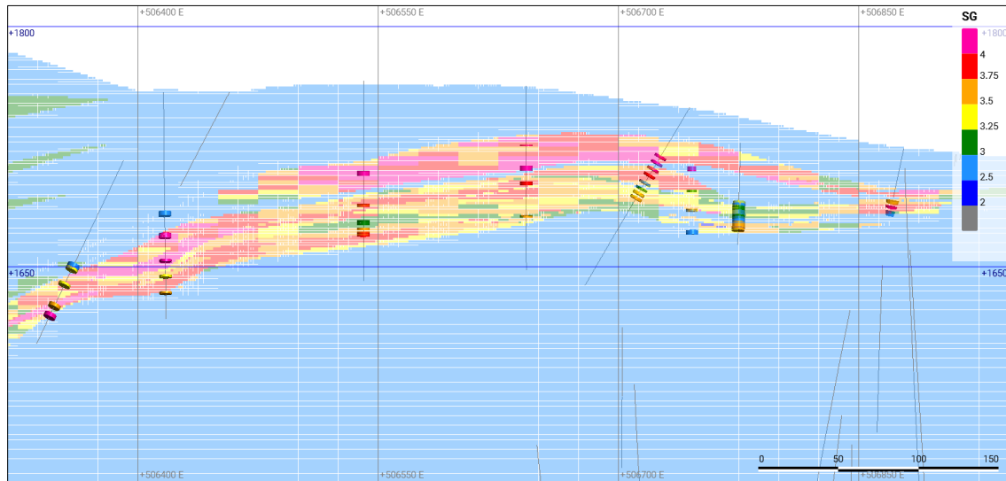
Figure 14.18 JL UCZ Section N5180805 ( \pm 17.5 m) Looking North at SG Block Model versus SG Composites
