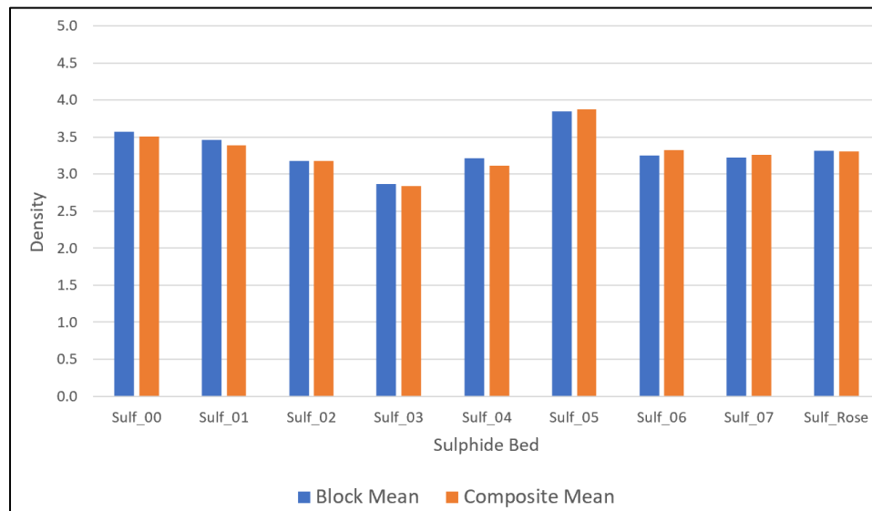
Figure 14.25 Comparison of Lowry Mean SG between Composites (orange) and Blocks (blue)
