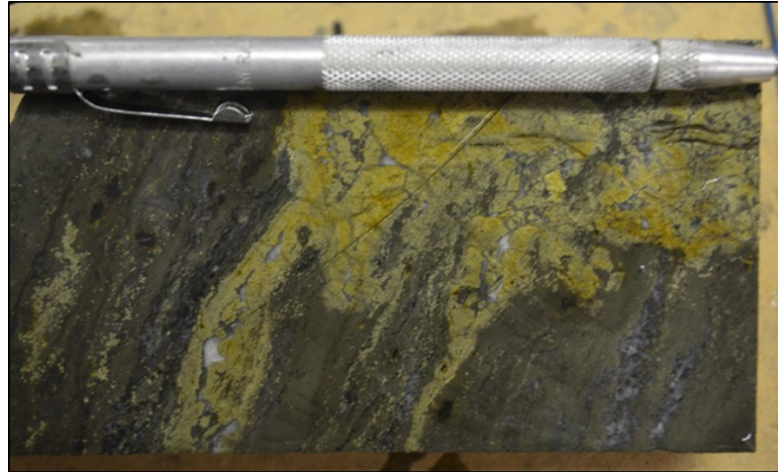
Figure 7.11 Coarse chalcopyrite veinlet cross-cutting layered bedded pyrite with narrow net textured layers in JL UCZ. Note the replacement along certain layers.
