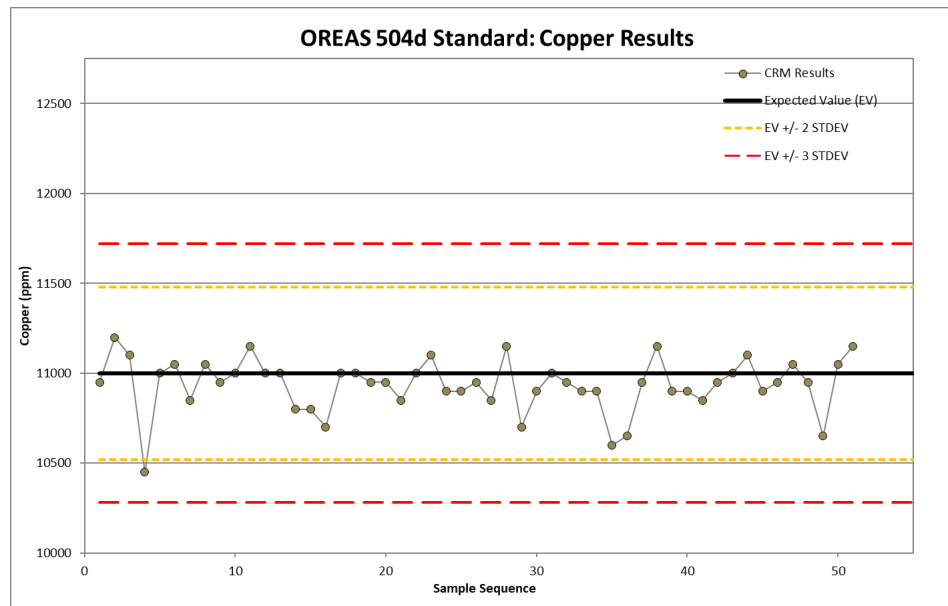
Figure 11.20 OREAS-504d Cu values from the 2023–2025 drill program
