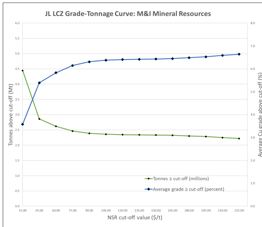
Figure 14.32 Grade-Tonnage Curve for the JL LCZ Main showing Measured and Indicated Mineral Resources
