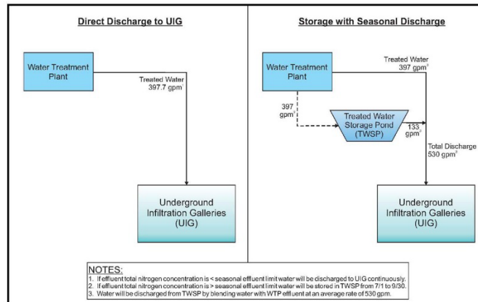
Figure 20.16 Average Annualized Water Balance During Mining Operations – Johnny Lee (part 2)
