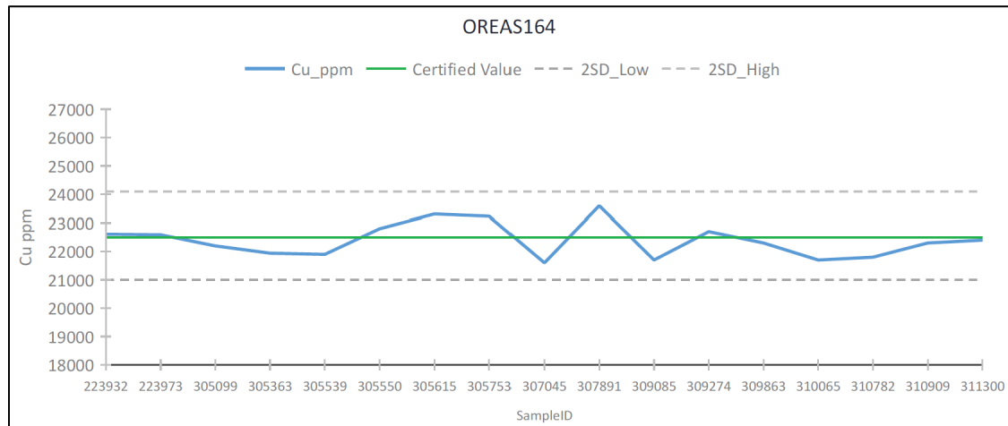
Figure 11.17 OREAS-164 Cu values from the 2021/22 drill program
