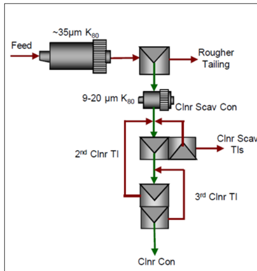
Figure 13.8 LCT's Flowsheet
