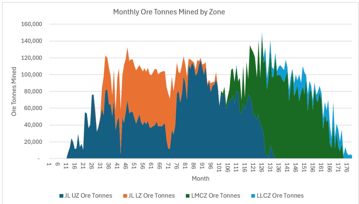
Figure 16.37 Monthly Ore Tonnes Mined by Zone (Entech, 2026)
