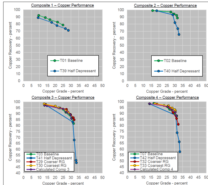
Figure 13.23 Reduced Depressant Results
