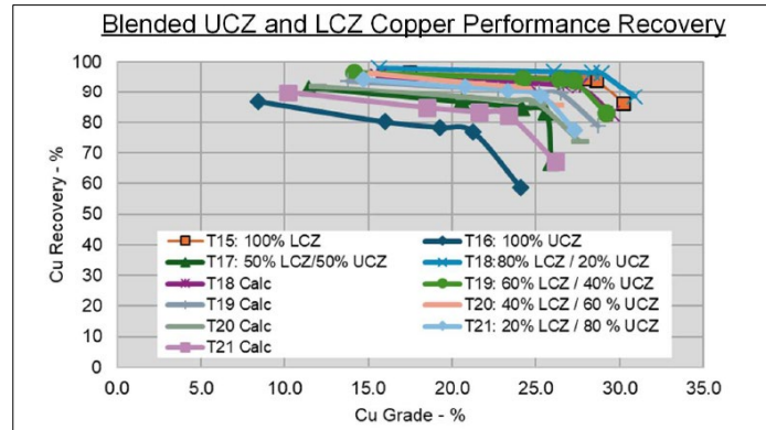
Figure 13.27 Copper Recovery for various blends
