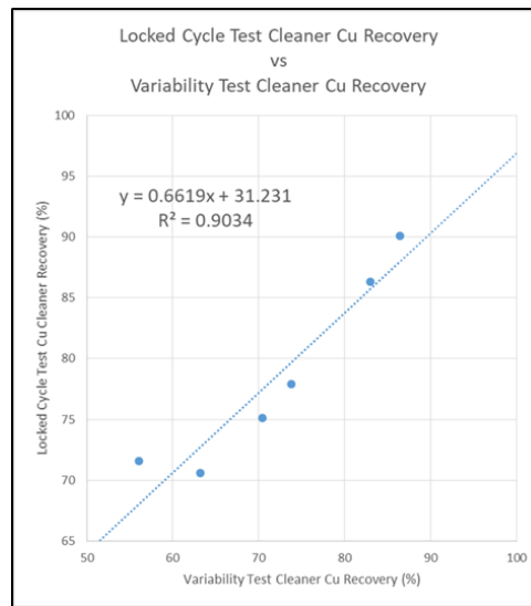
Figure 13.30 LCT Cleaner Recovery vs Variability Test Cleaner Recovery
