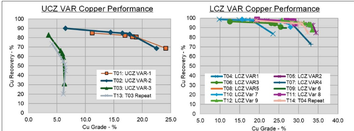
Figure 13.26 Copper Recovery for Variability Samples (JL UCZ and JL LCZ)
