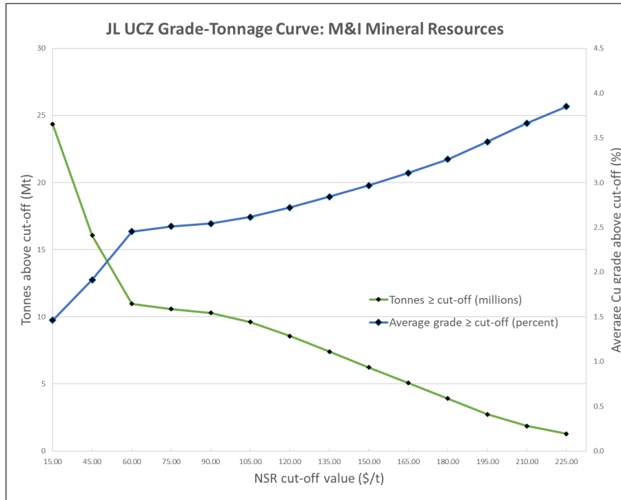
Figure 14.31 Grade-Tonnage Curve for the JL UCZ showing Measured and Indicated Mineral Resources
