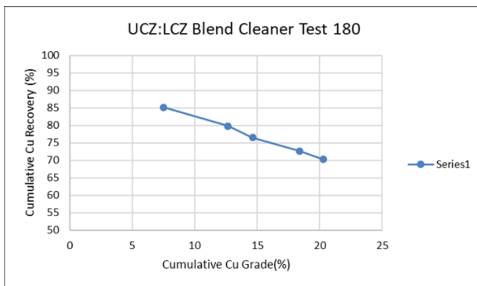
Figure 13.11 JL UCZ - JL LCZ Batch Cleaner Test (T-180)
