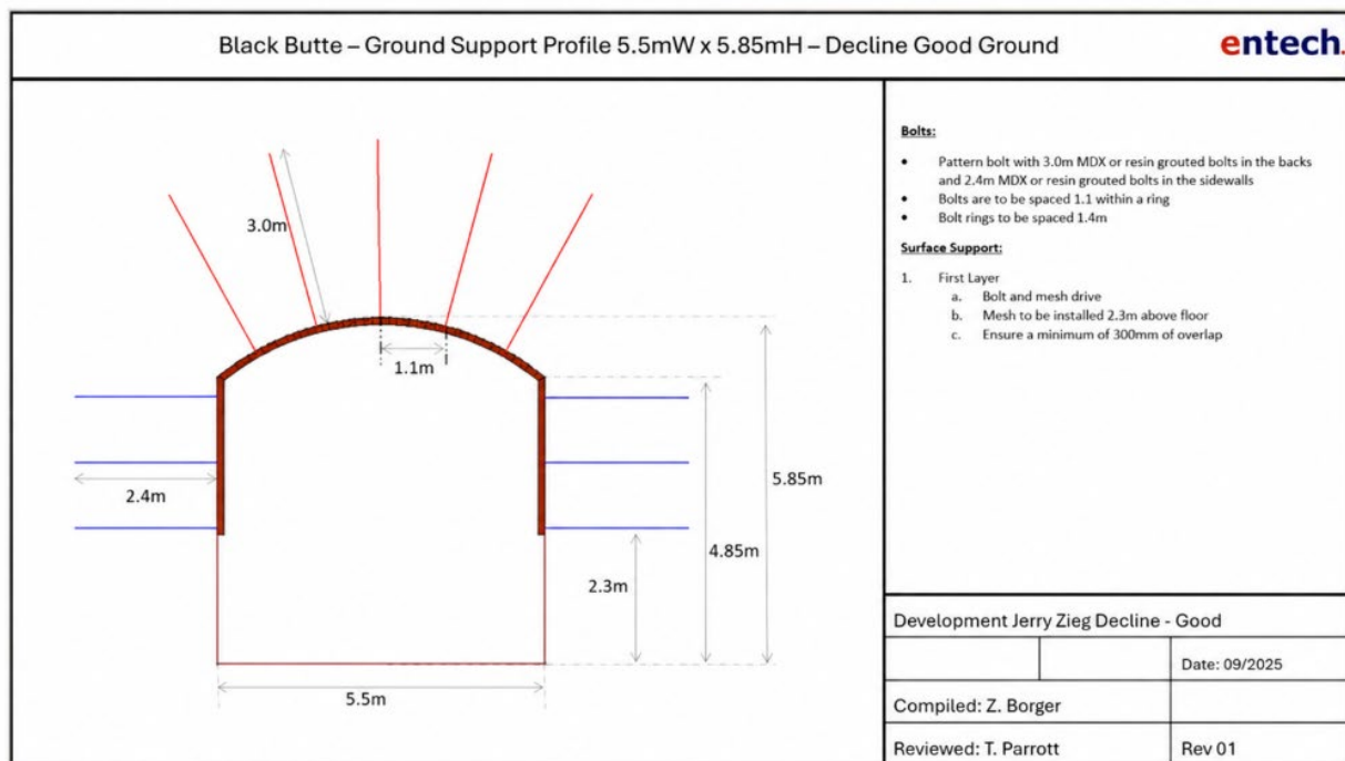
Figure 16.17 12 Ground support layout for Jerry Zieg Decline development - Good Ground (Entech, 2026)
