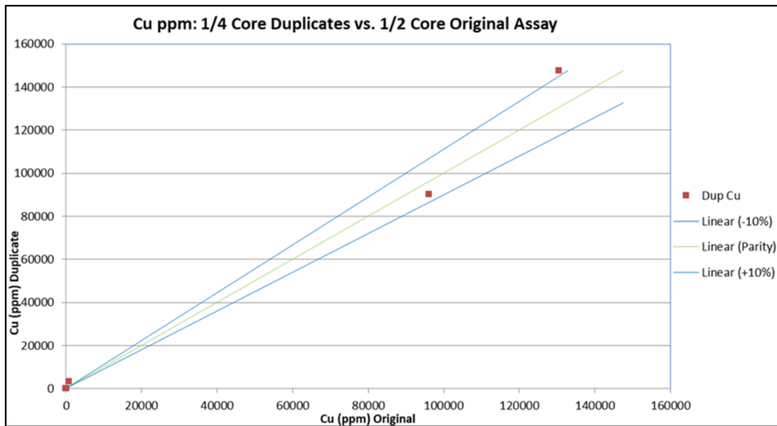
Figure 11.34 Comparison of Cu analyses from original and field duplicates from the 2018 Phase 1 drill program
