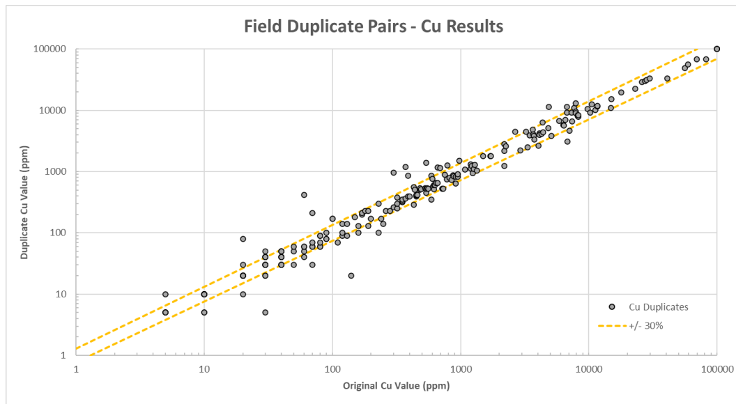
Figure 11.39 Comparison of Cu analyses from original and field duplicates for the 2023–2025 drill program
