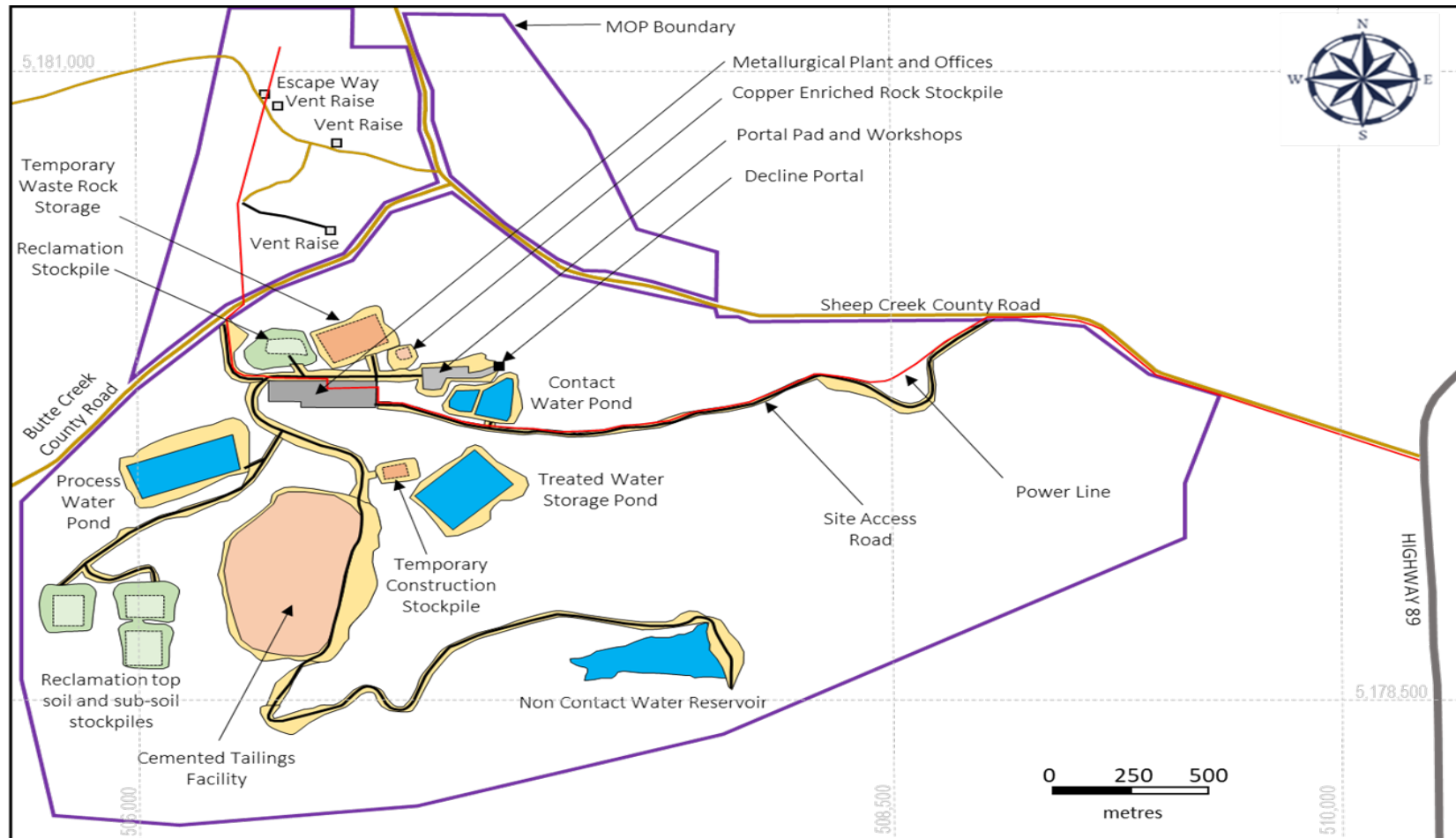
Figure 5.2 Proposed Infrastructure Layout for the Black Butte Copper Project
