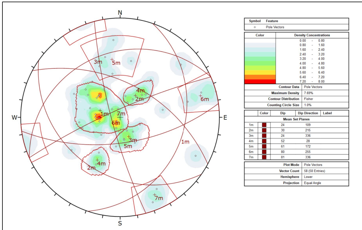
Figure 16.13 9 Stereonet plot displaying orientated structure for the LCZ at Johnny Lee (Entech, 2026)
