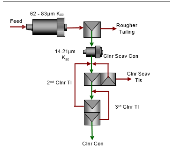
Figure 13.15 LCT Flowsheet
