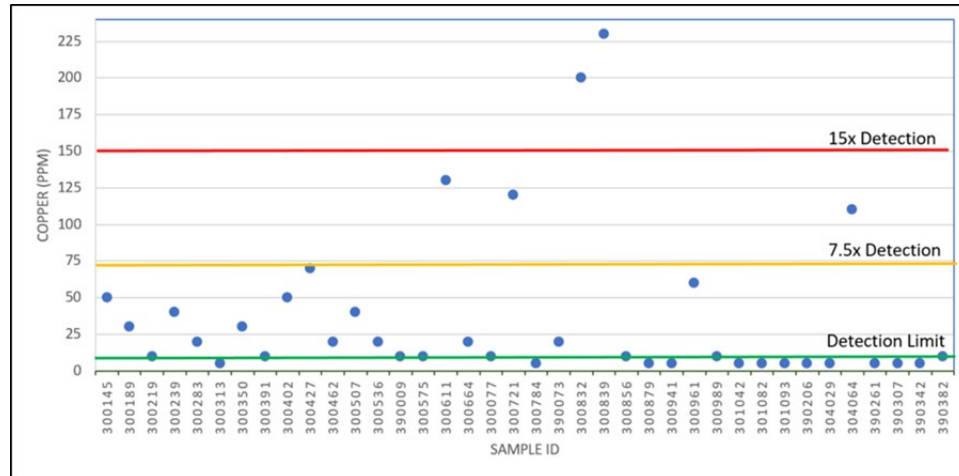
Figure 11.29 Cu results for coarse blanks for the 2018/19 Phase 2 drill program
