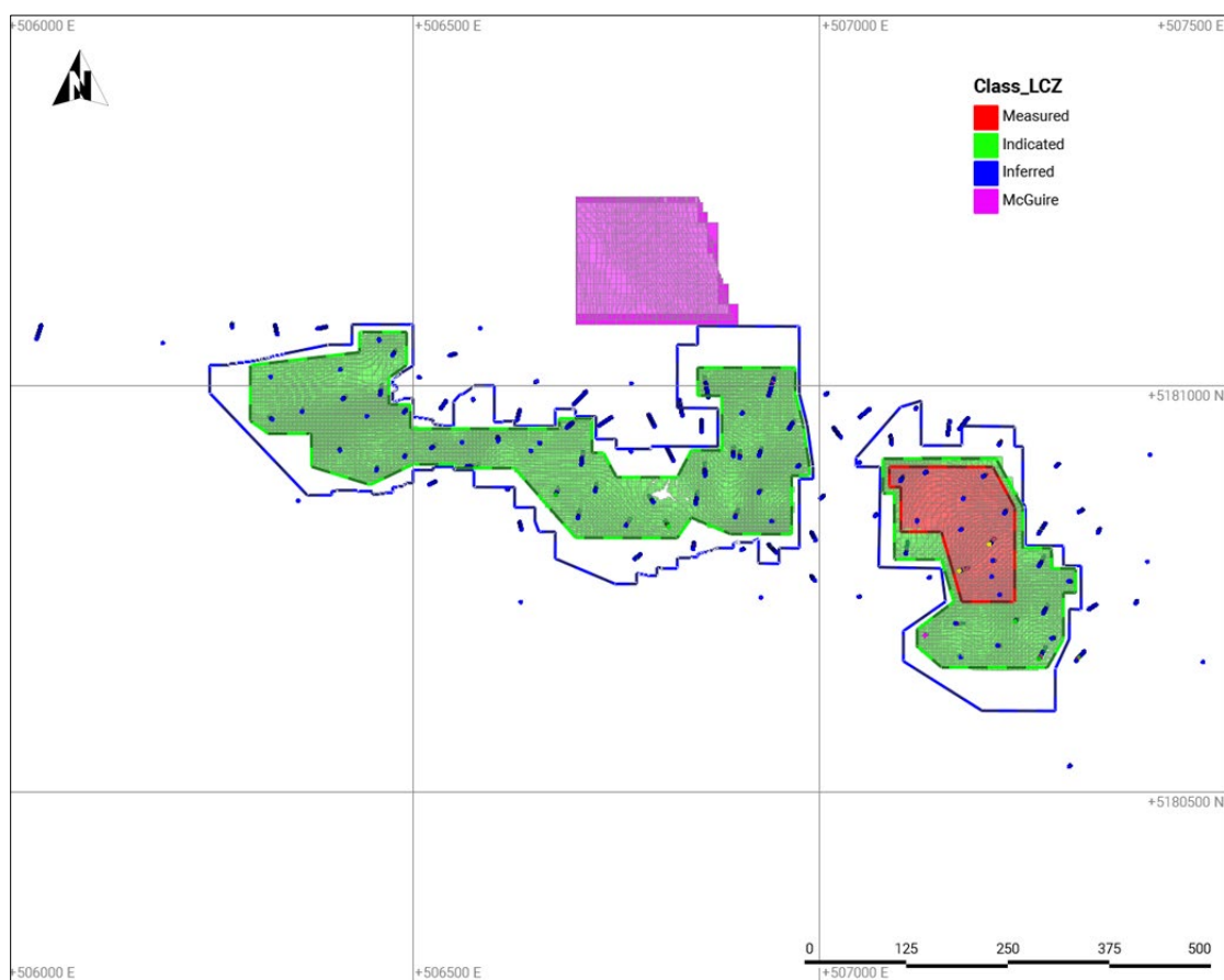
Figure 14.28 Plan View of the JL LCZ showing Mineral Resource Classification
