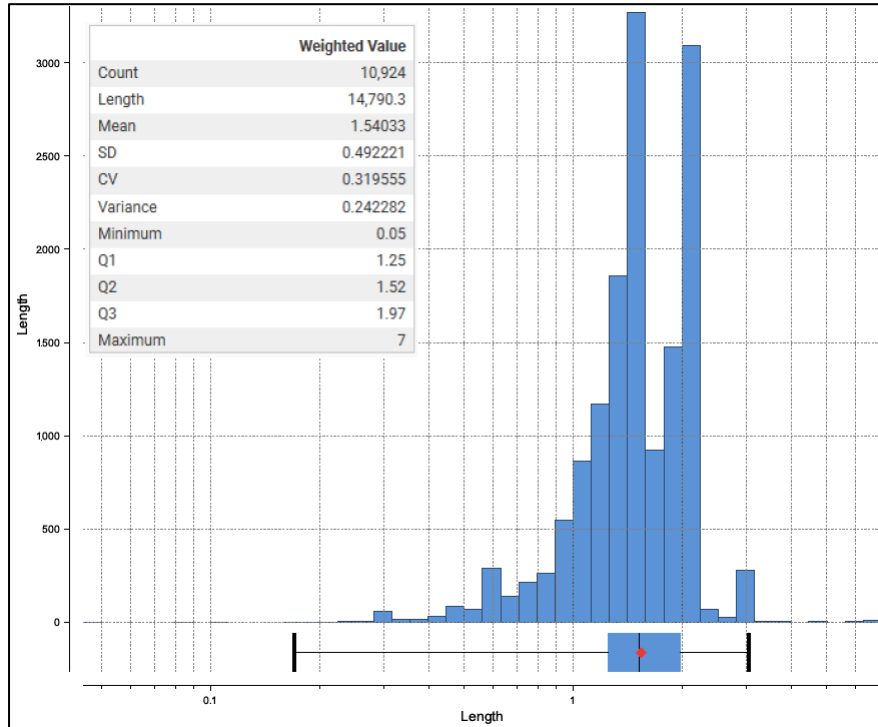
Figure 14.11 Histogram of Sample Lengths in the Lowry deposit
