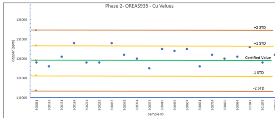
Figure 11.11 OREAS-935 Cu values from the 2018/19 Phase 2 drill program
