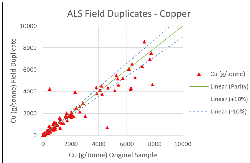
Figure 11.38 Comparison of Cu analyses from original and field duplicates for the 2021/22 drill program
