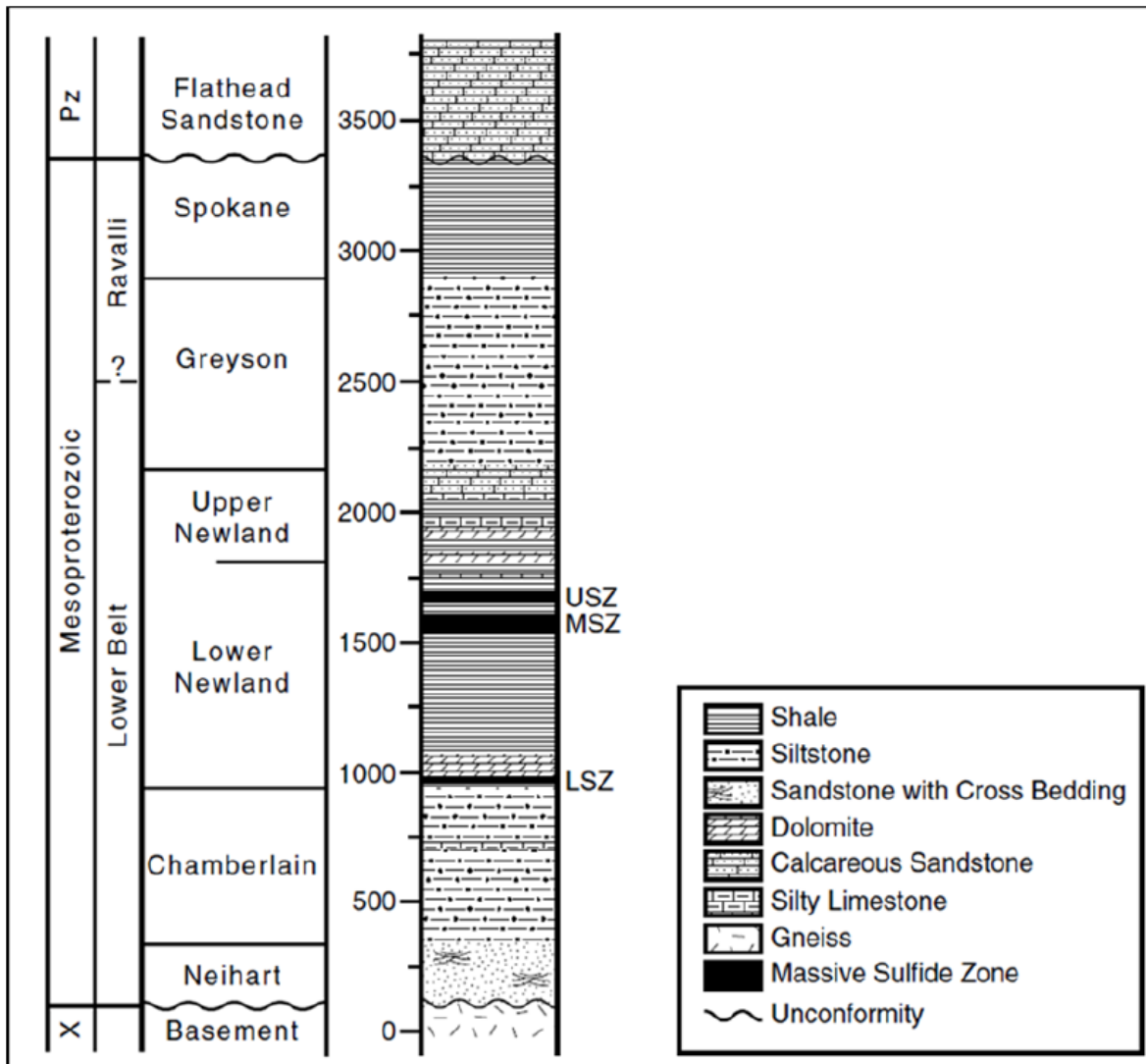
Figure 16.5 3 Project area stratigraphy with thickness scale (Source: Tintina Resources Ltd)
