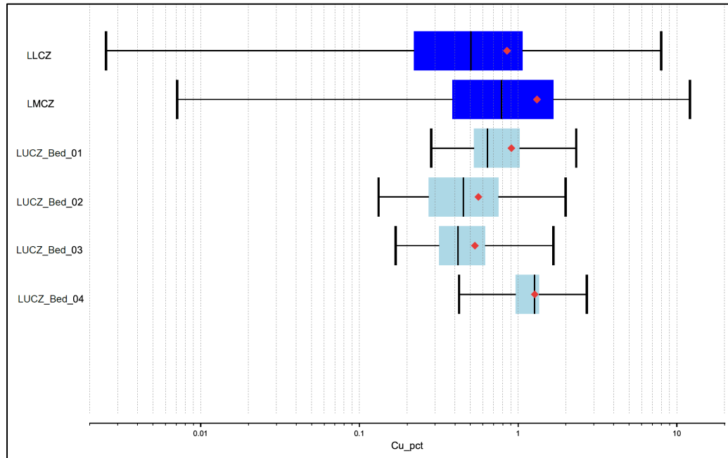
Figure 14.14 Box and Whisker Plot of Cu grades (log scale) within the Lowry grade shapes
