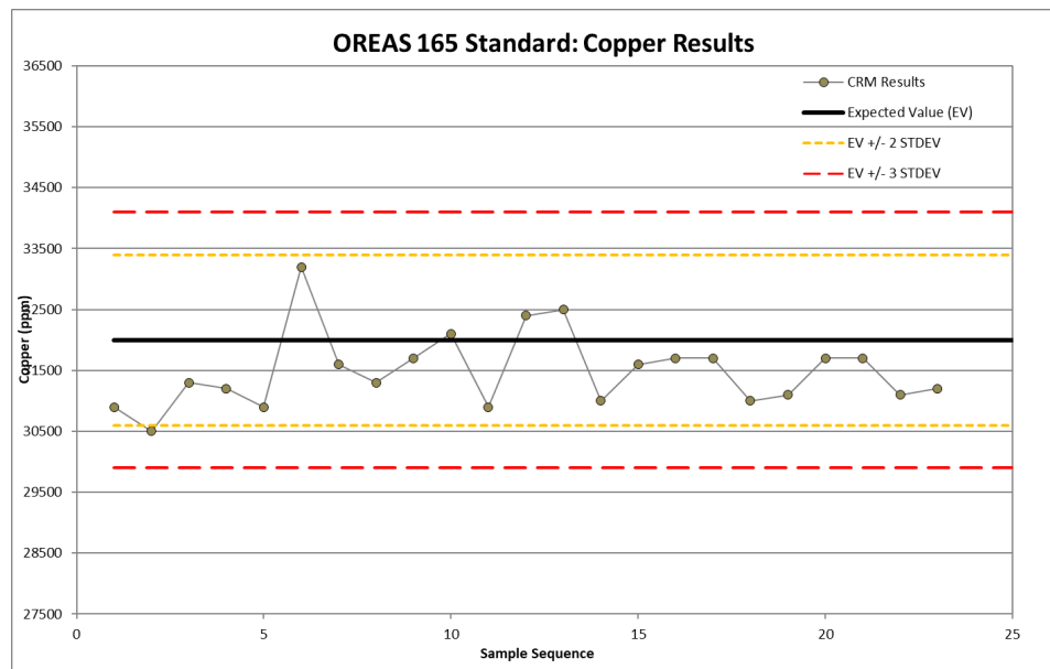
Figure 11.19 OREAS-165 Cu values from the 2023–2025 drill program
