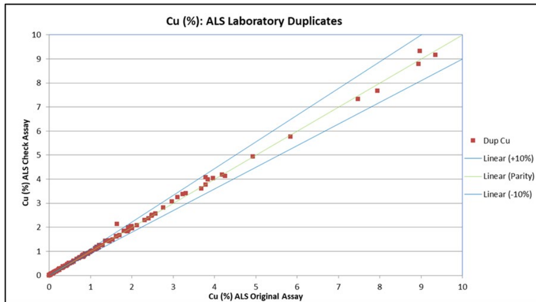
Figure 11.36 Scatter plot of laboratory duplicate Cu analyses for the 2018/19 Phase 2 drill program.
