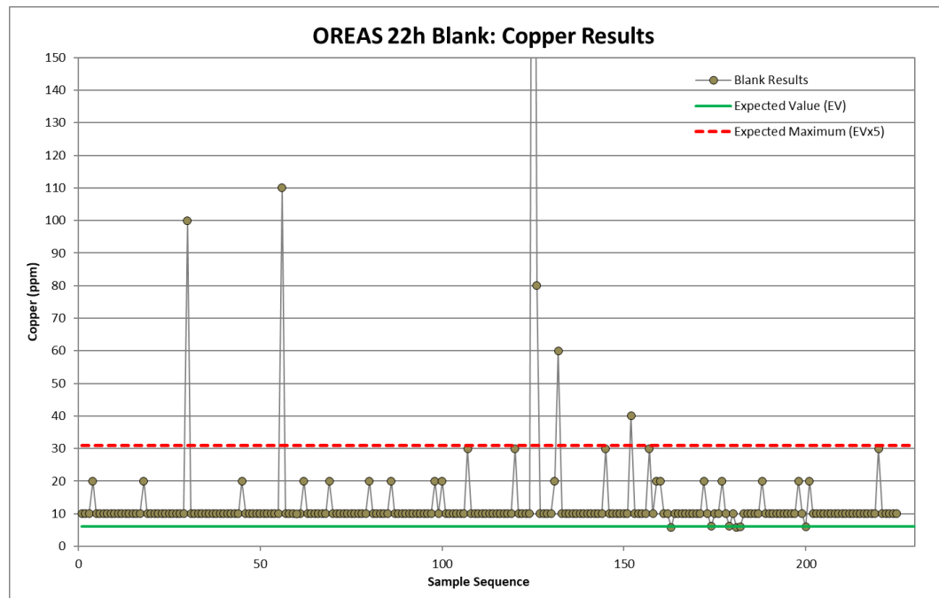
Figure 11.32 Cu results for OREAS-22h blanks over the 2023–2025 drill program
