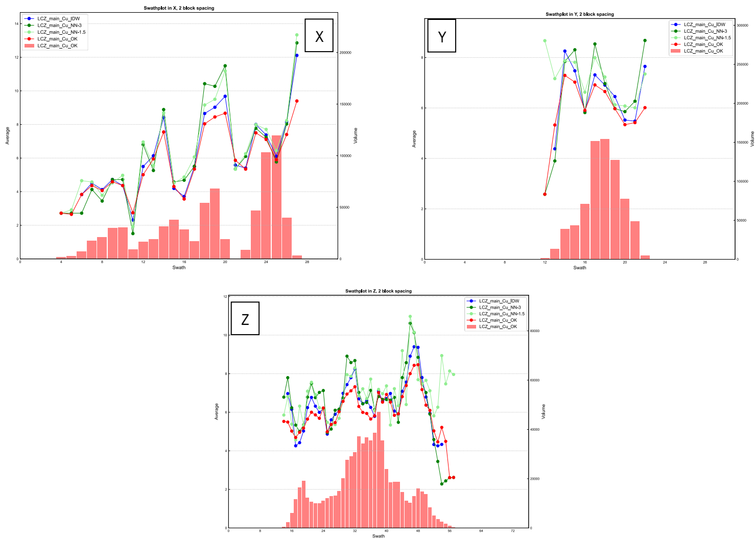
Figure 14.22 JL LCZ Main Swath Plots
