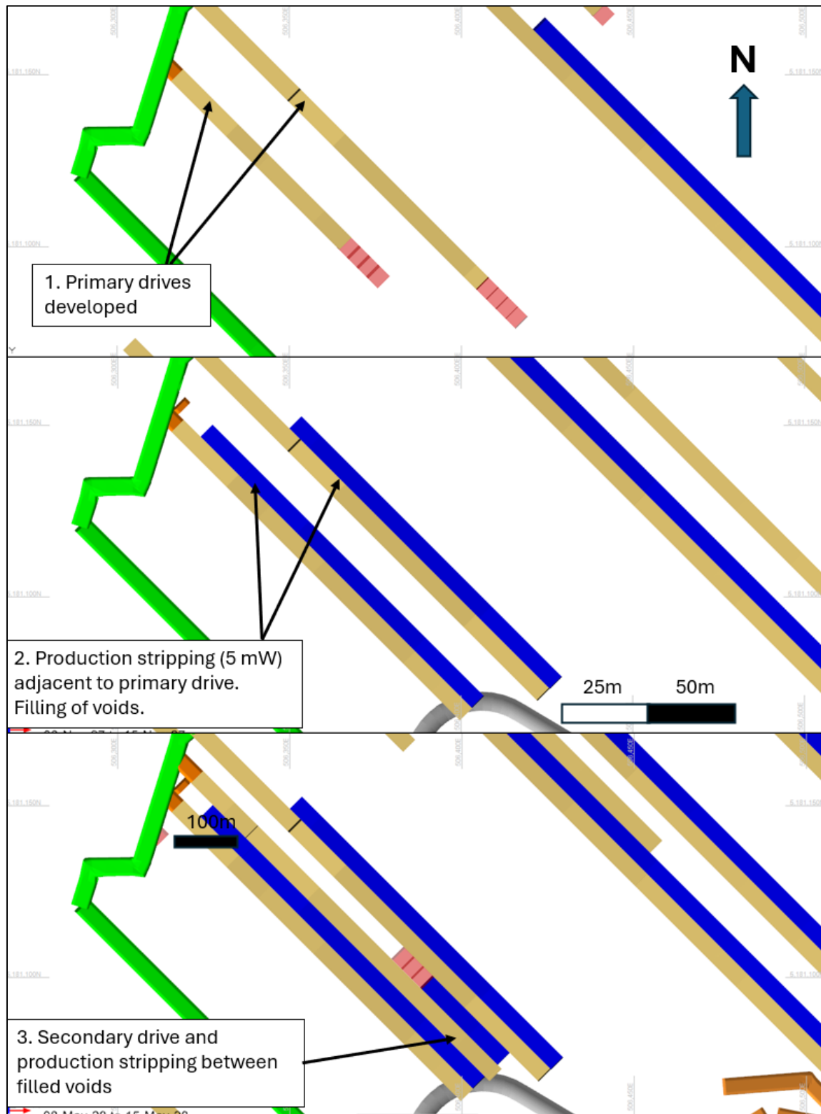
Figure 16.25 JL UCZ Production Mining Sequence (Plan View) (Entech, 2025)
