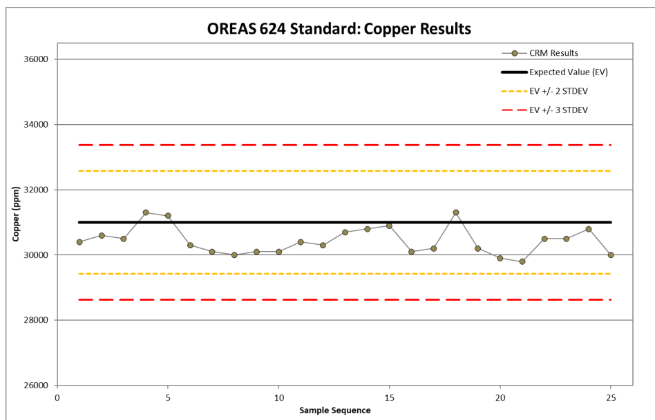
Figure 11.21 OREAS-624 Cu values from the 2023–2025 drill program
