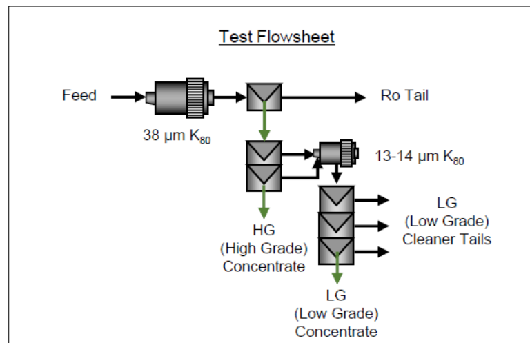
Figure 13.24 Alternative Cleaner Flowsheet
