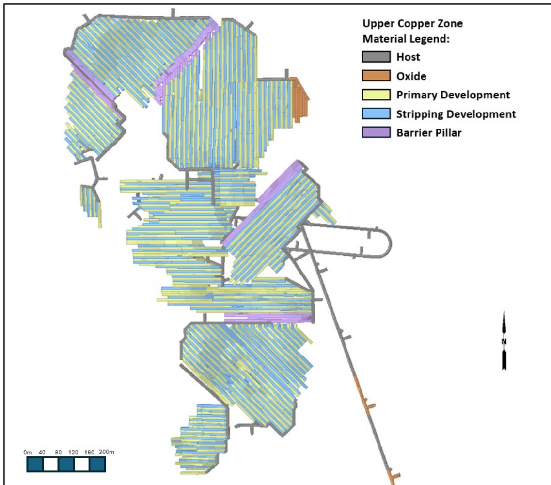
Figure 16.16 11 Plan view of UCZ at Johnny Lee showing placement of Barrier Pillars within the mine design (Entech, 2026)
