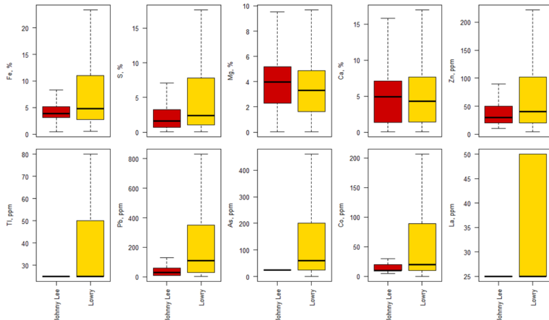
Figure 20.13 Boxplots of select parameters from multi-element testing of the Ynl waste rock in the Johnny Lee (JL) and Lowry (L) deposits. (RESPEC, 2026)
