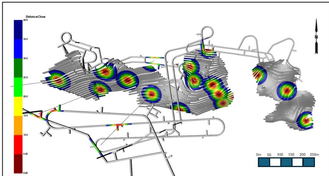
Figure 16.2 Plan view Geotechnical drill hole coverage for Johnny Lee LCZ with a heat map extrapolated 40 m (Entech, 2025)
