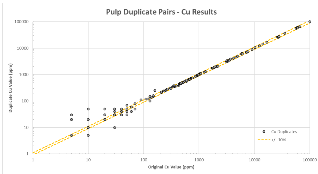
Figure 11.40 Comparison of laboratory pulp duplicate Cu analyses for the 20232025 drill program
