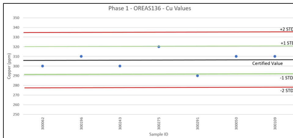
Figure 11.10 OREAS-136 Cu values from the 2018 Phase 1 drill program
