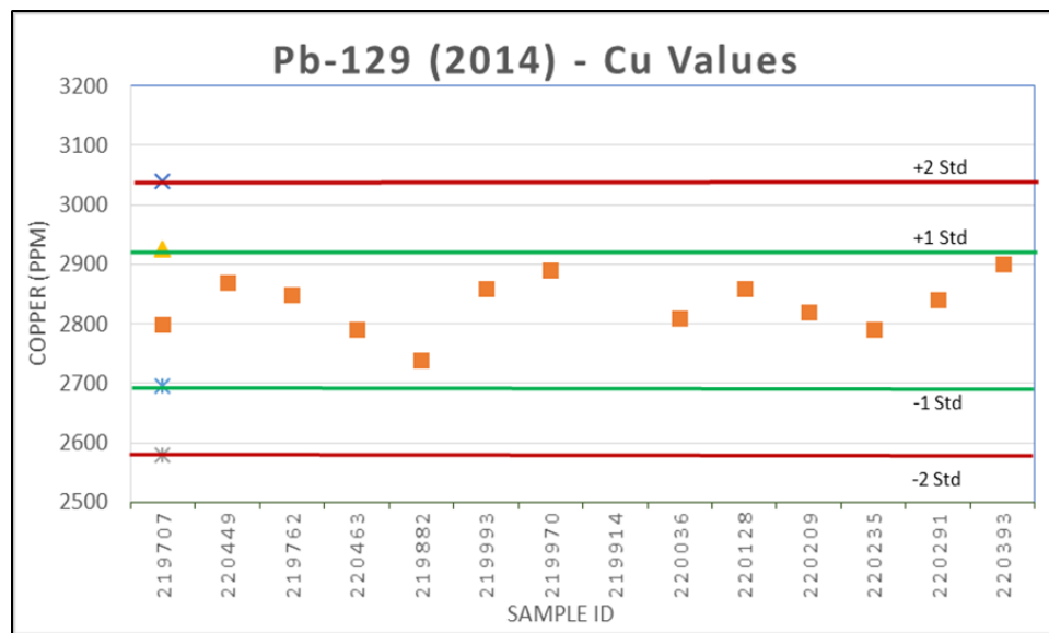
Figure 11.6 Pb-129 Cu values from 2014 drill program
