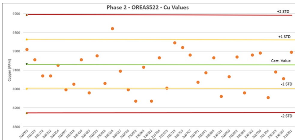
Figure 11.13 OREAS-522 Cu values from the 2018/19 Phase 2 drill program
