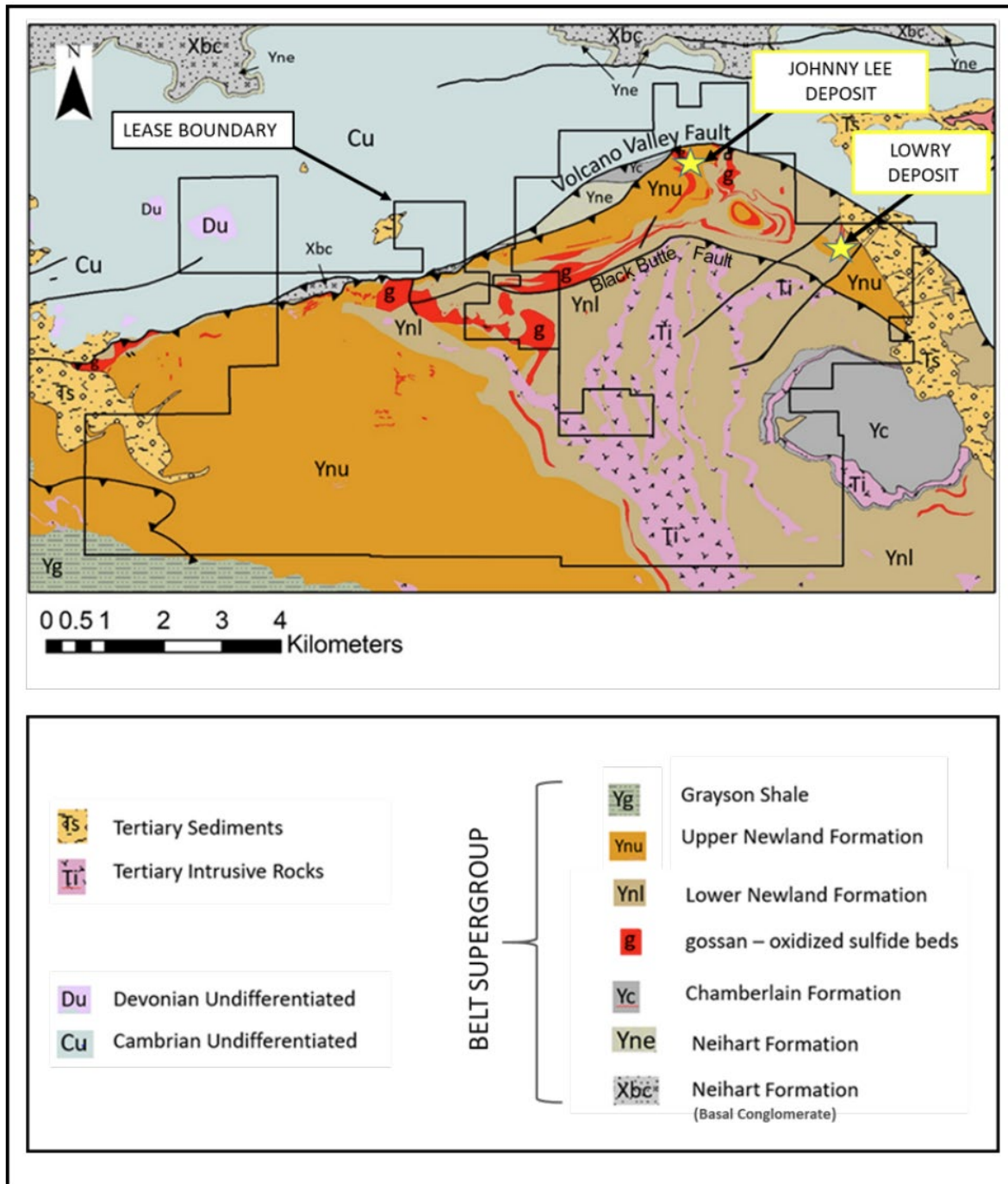
Figure 16.4 2 Regional Geological Map of Black Butte Copper Project Site (Source: Tintina Resources Ltd)
