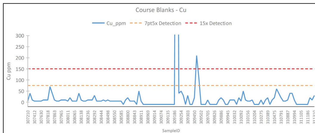
Figure 11.30 Cu results for coarse blanks for the 2021/22 drill program
