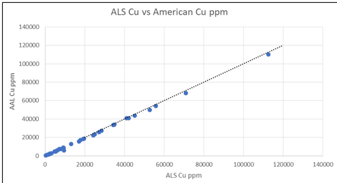
Figure 11.35 Comparison between AAL umpire and ALS original Cu assays for the 2018 Phase 1 drill program
