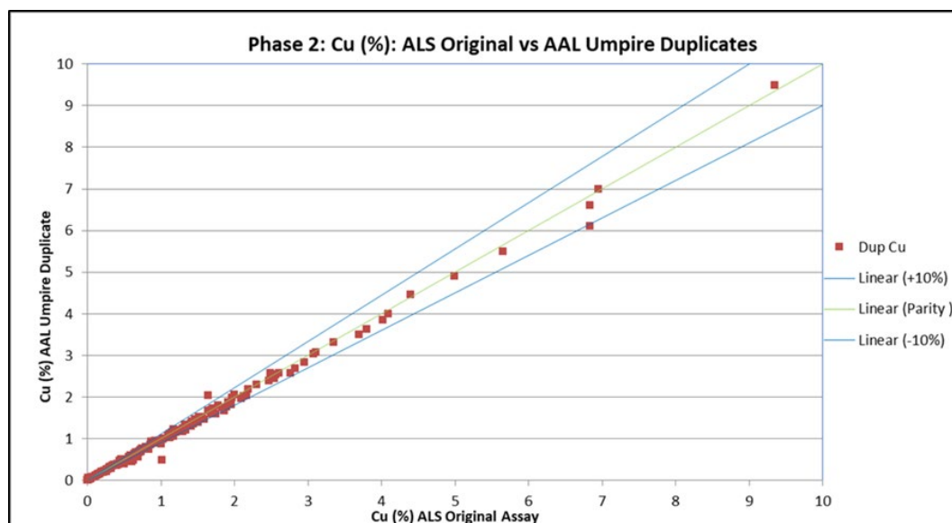
Figure 11.37 Scatter plot of umpire duplicate copper analyses for the 2018/19 Phase 2 drill program
