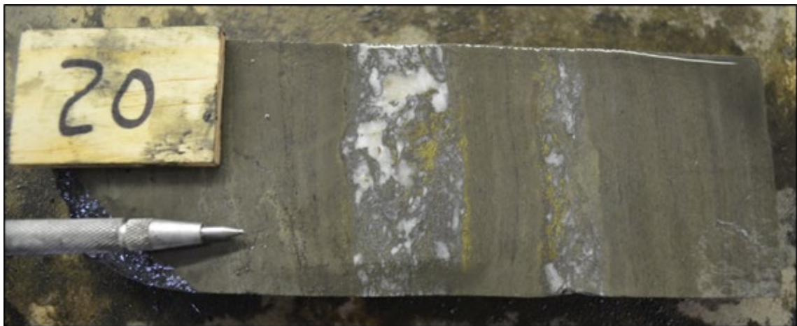
Figure 7.12 Preferential replacement of net-textured layers with chalcopyrite within bedded pyrite of the JL UCZ
