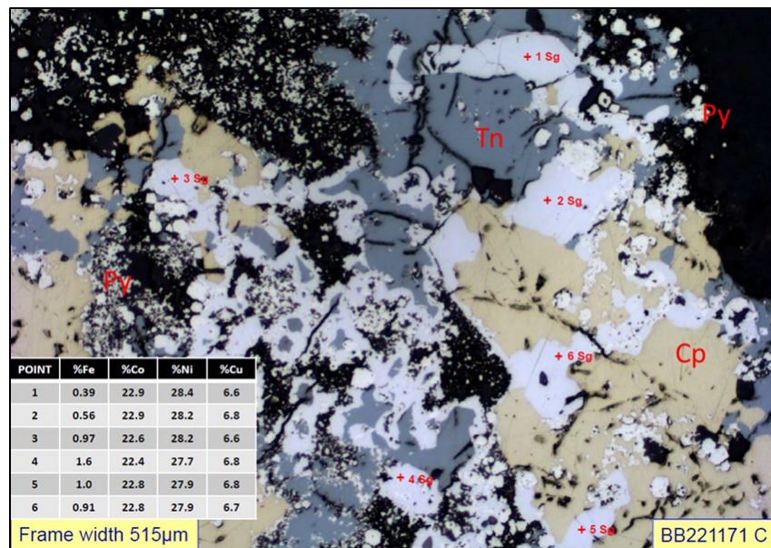
Figure 7.21 Reflected light photomicrograph of a JL UCZ ore sample showing microprobe analyses points for cuprian siegenite (sg) and analytical results. Tn = tennantite, Cp = chalcopyrite, Py = pyrite. (McArthur, 2018)
