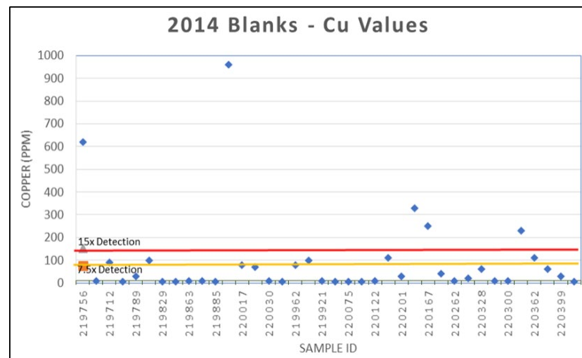
Figure 11.26 Cu results of landscape marble used as coarse blanks during the 2014 drill program
