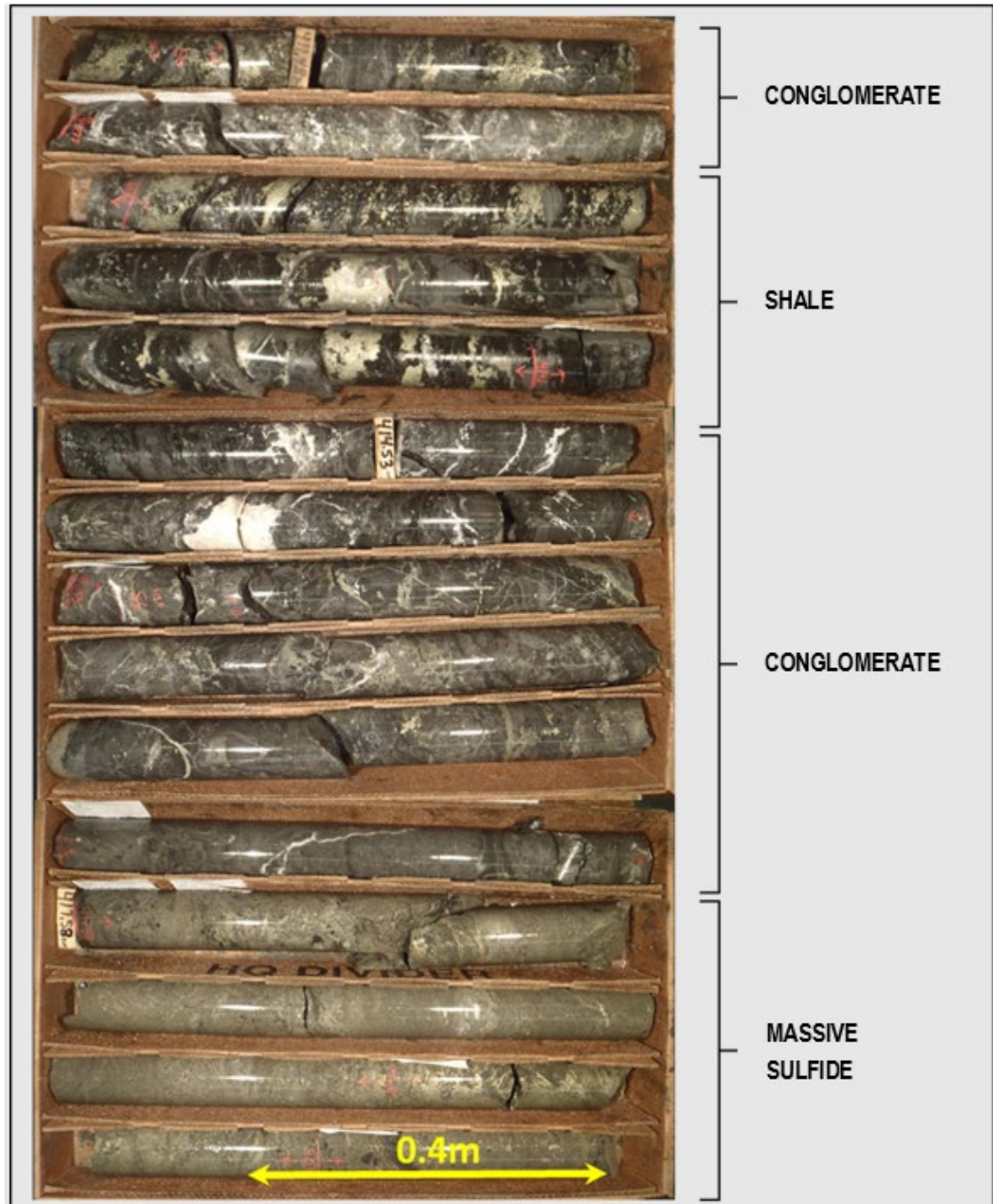
Figure 7.9 Core photographs of drillhole SC11-011 from 411.2 m (top) to 419.7 m (base) showing chalcopyrite hosted Cu mineralization extending from massive sulfide of the JL LSZ into interlayered shale and conglomerate
