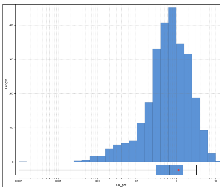
Figure 14.13 Histogram of Composited Cu grades within the LMCZ and LLCZ
