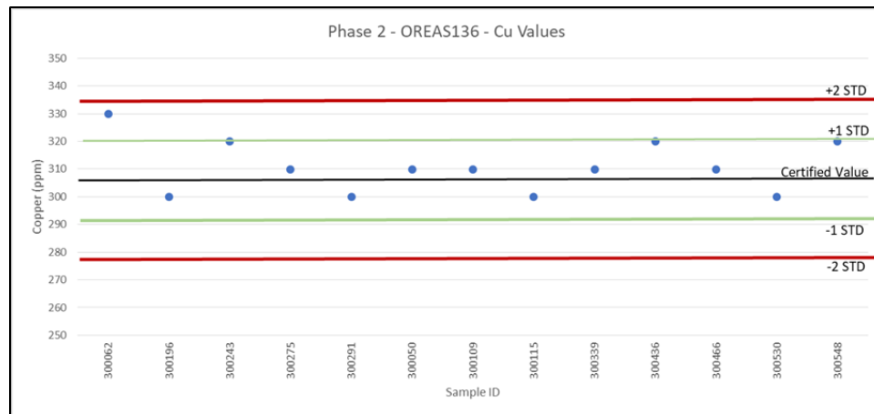
Figure 11.15 OREAS-136 Cu values from the 2018/19 Phase 2 drill program
