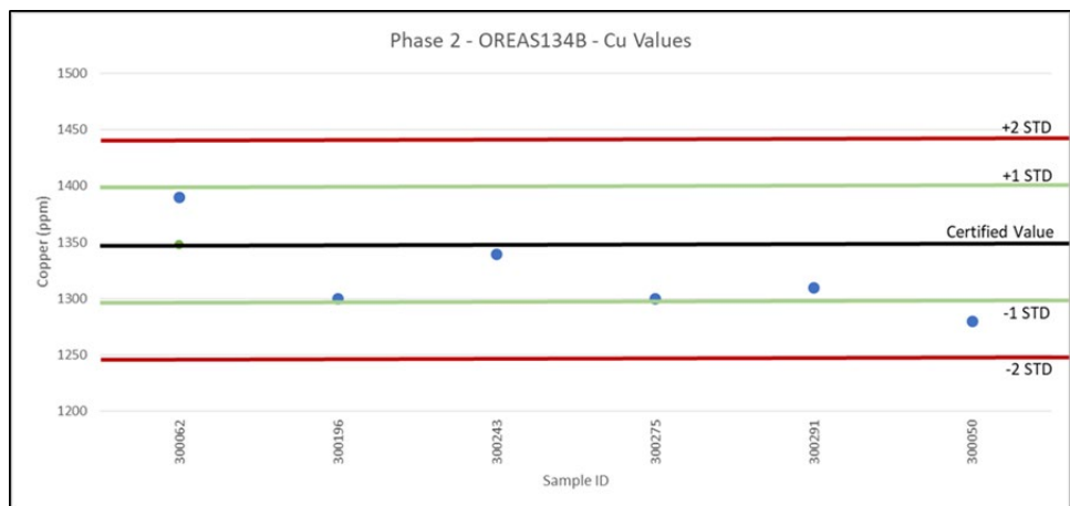
Figure 11.14 OREAS-134B Cu values from the 2018/19 Phase 2 drill program
