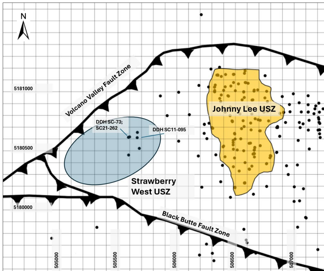
Figure 9.4 Plan view showing the Strawberry West prospect area and the locations of the VVFZ, BBF, and Johnny Lee USZ and drillhole collar locations
