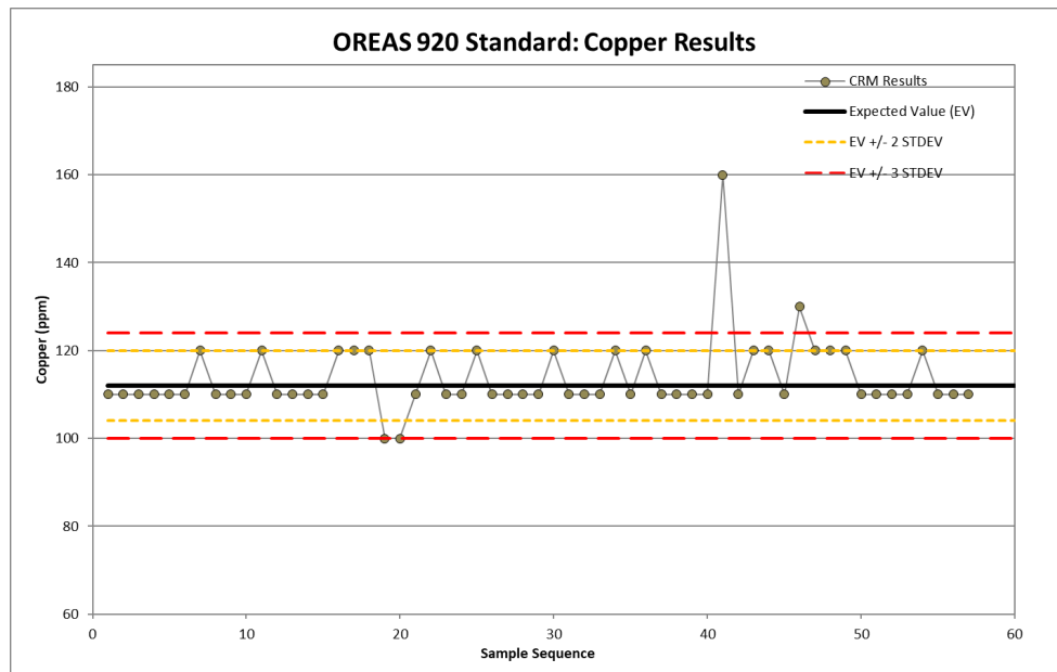
Figure 11.22 OREAS-920 Cu values from the 2023–2025 drill program
