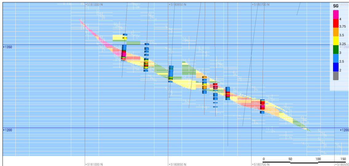
Figure 14.19 JL LCZ Section E507220 ( \pm 22.5 m) Looking East at SG Block Model versus SG Composites
