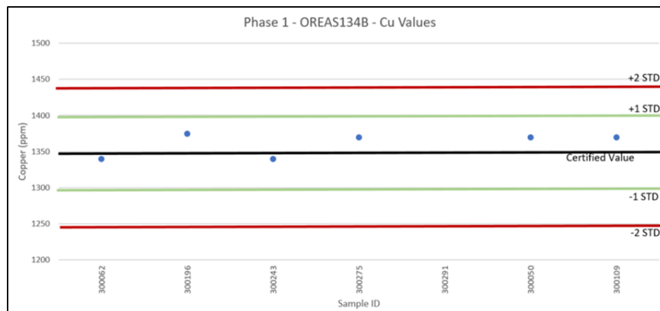
Figure 11.9 ORES-134B Cu values from the 2018 Phase 1 drill program
