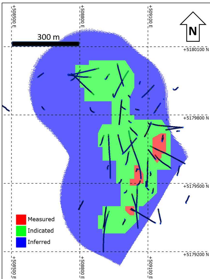
Figure 14.30 Plan View of the LLCZ showing Mineral Resource Classification
