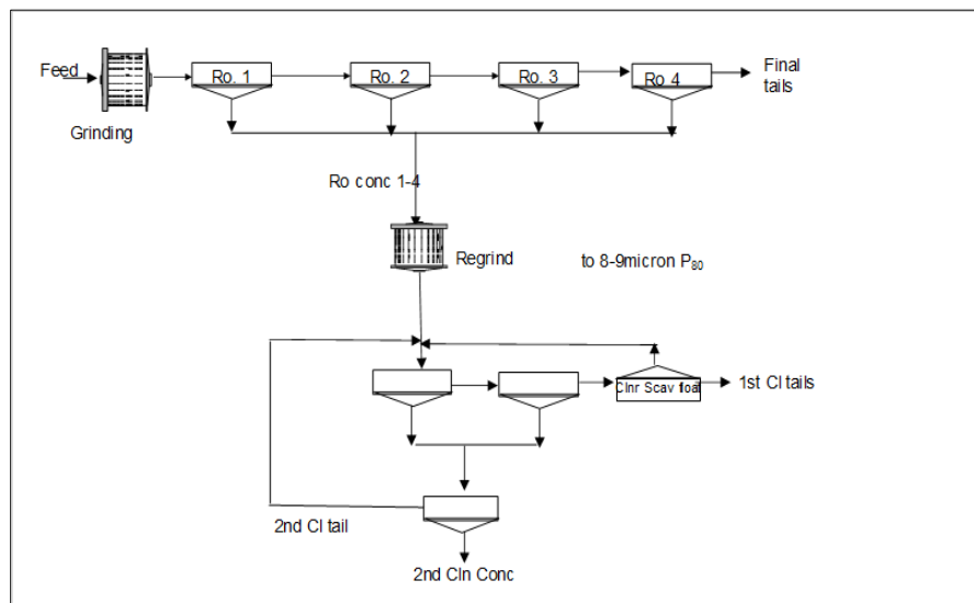
Figure 13.4 LCT Flowsheet for LCZ
