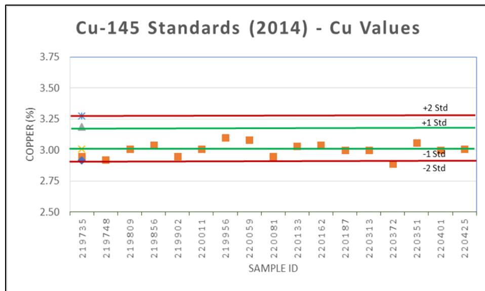
Figure 11.4 Cu-145 Cu values from the 2014 drill program
