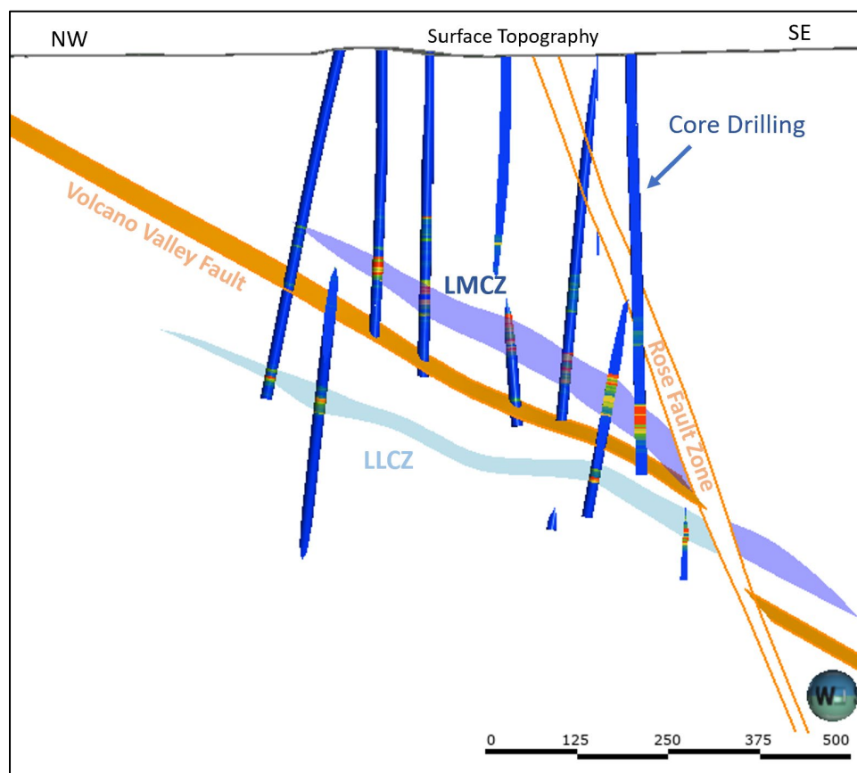
Figure 14.5 Cross-section of the LMCZ & LLCZ along line NW-SE (Figure 14.4) looking northeast
