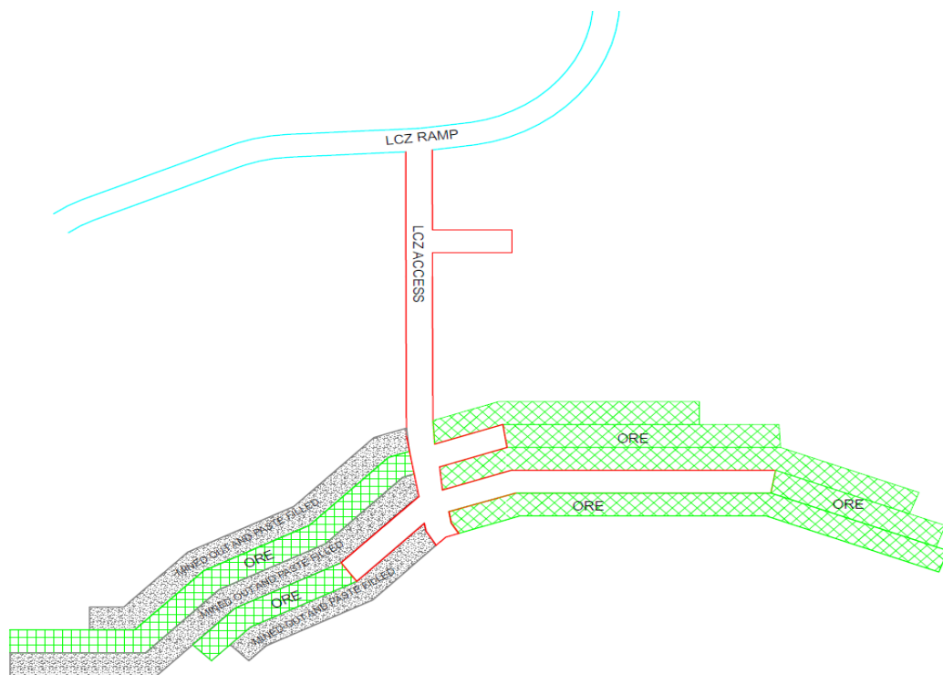
Figure 16.26 Plan View Schematic JL LCZ Ore Extraction (SRA 2022)
