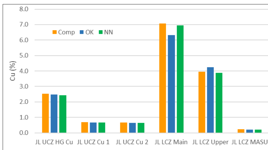
Figure 14.20 Comparison of JL Mean Cu Grades for Composites (orange), OK Blocks (blue), and NN Blocks (Green)
