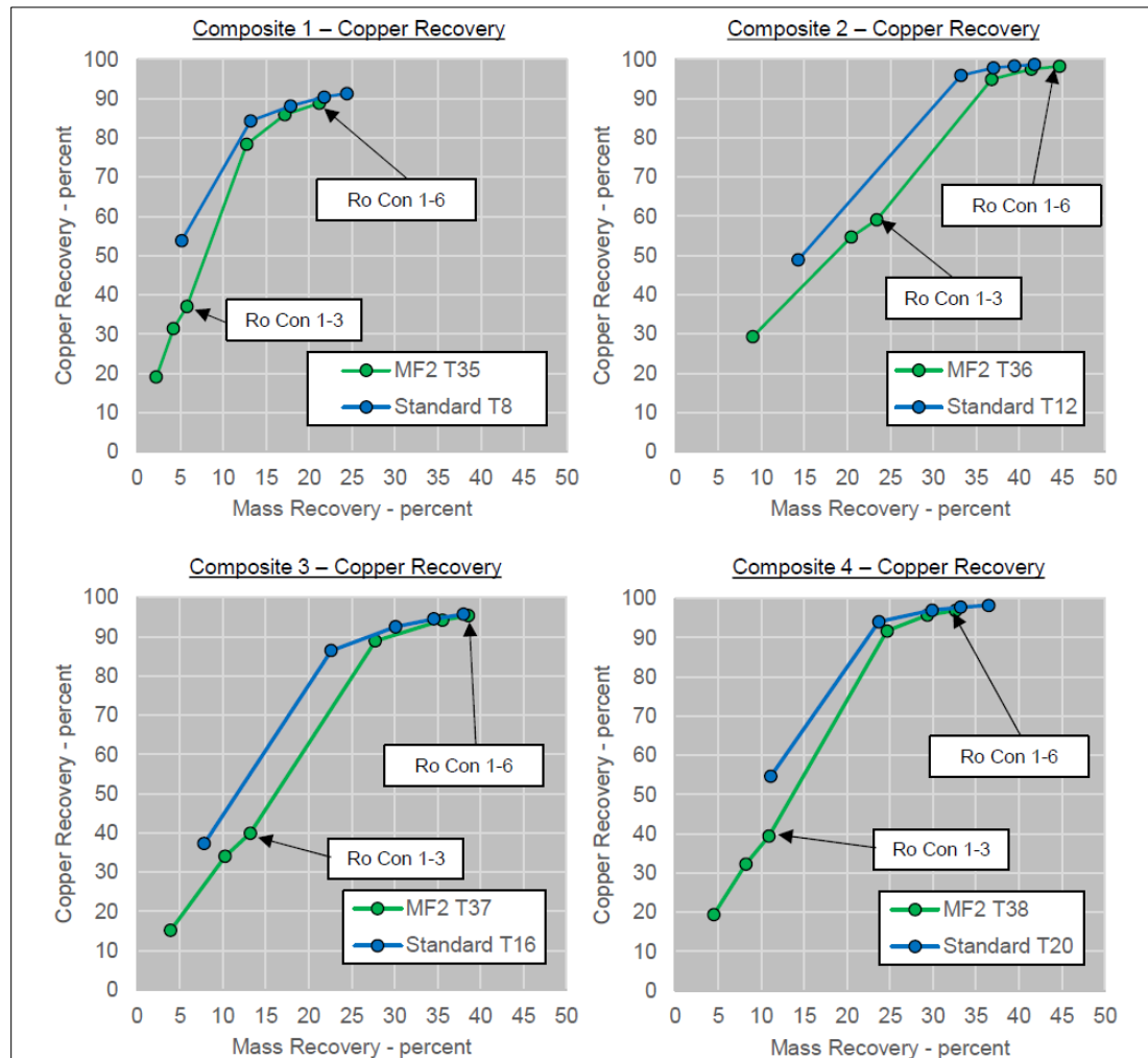
Figure 13.20 MF2 Copper Recovery Results
