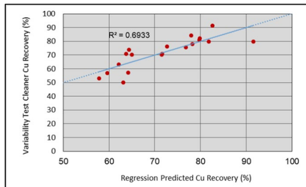
Figure 13.29 Cu Cleaner vs Regression Cu Recovery
