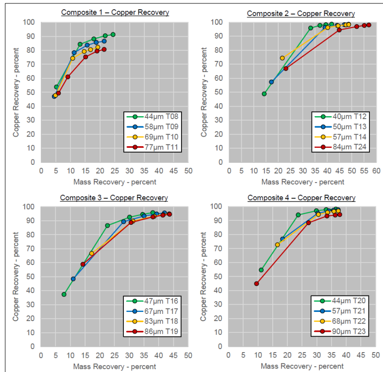
Figure 13.18 Grind Size Optimization – Rougher Stage
