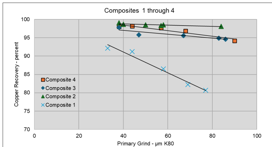
Figure 13.17 Copper recovery vs Grind Size for 4 composites
