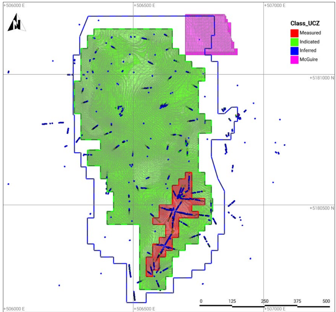
Figure 14.27 Plan View of the JL UCZ showing Mineral Resource Classification
