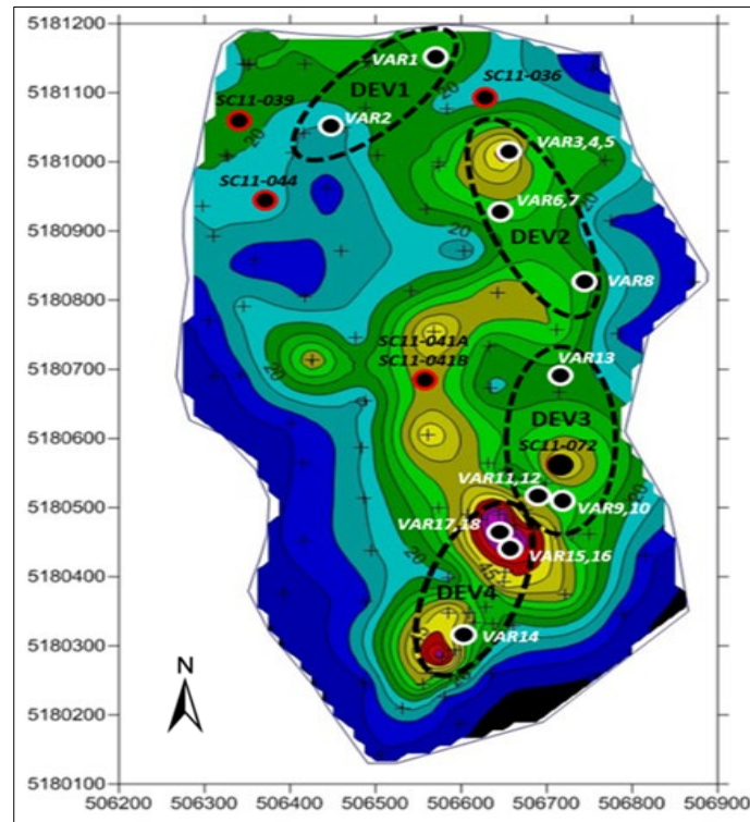
Figure 13.1 PEA And PFS Sample Location Map
