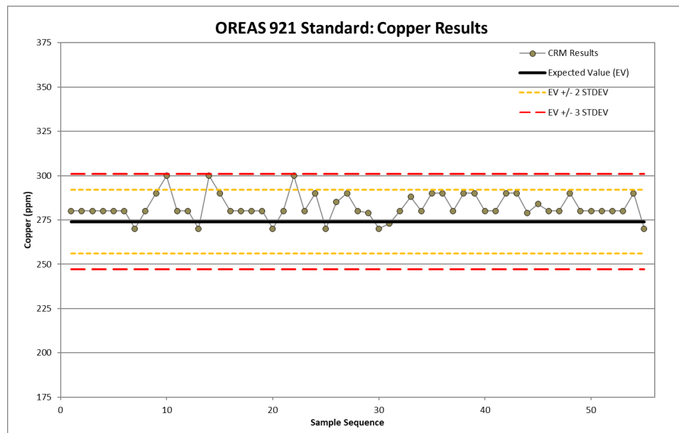
Figure 11.23 OREAS-921 Cu values from the 2023–2025 drill program
