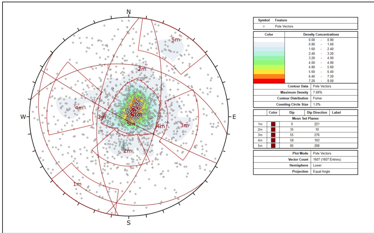
Figure 16.11 7 Stereonet plot displaying orientated structure data for Johnny Lee deposit (Entech, 2026)
