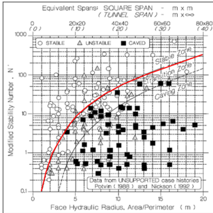
Figure 16.15 10 Potvin Stability Graph for Stable Unsupported Stope Spans. The red line indicates the Stable Unsupported Limit for which stope spans have been designed upon (Potvin, 1988)
