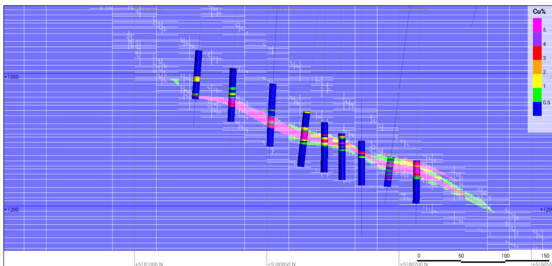
Figure 14.17 JL LCZ Section E507220 ( \pm 22.5 m) Looking East at Cu Block Model versus Cu Composites
