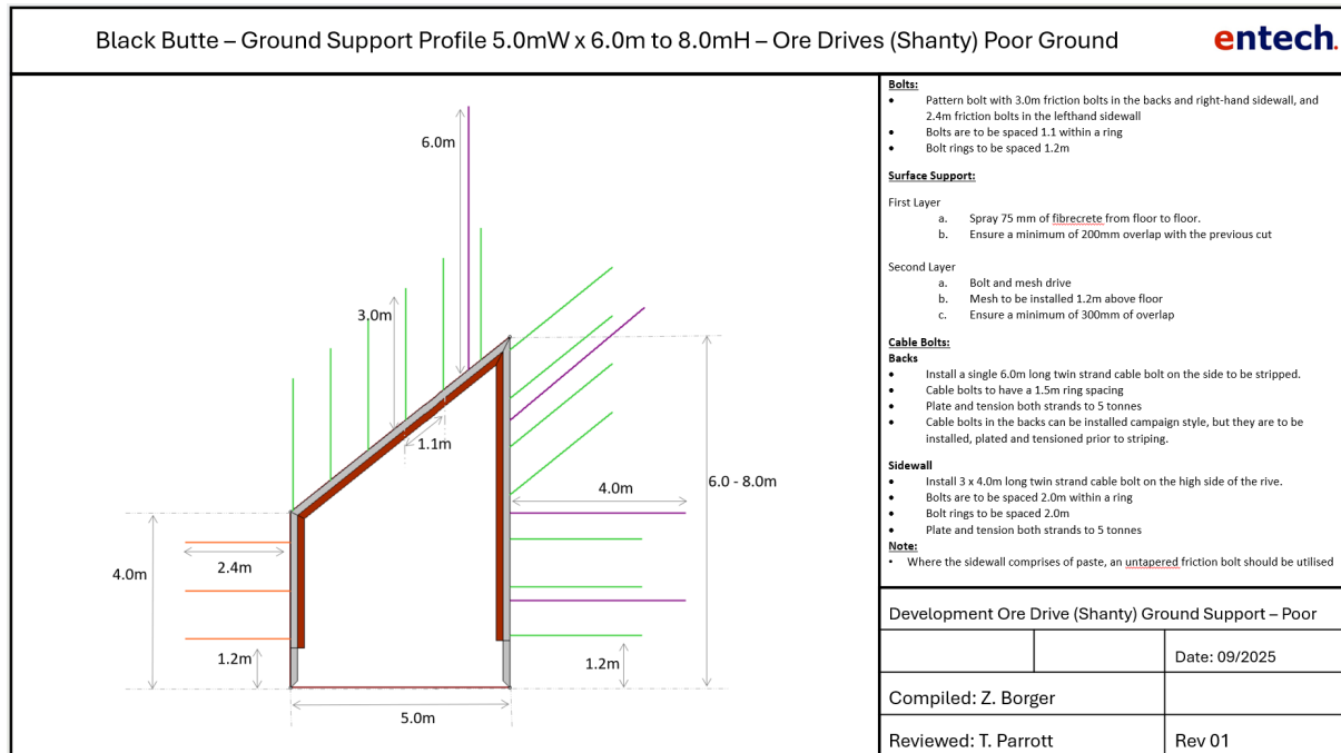
Figure 16.20 Ground support layout for ore drive development in LSZ - poor ground (Entech, 2026)
