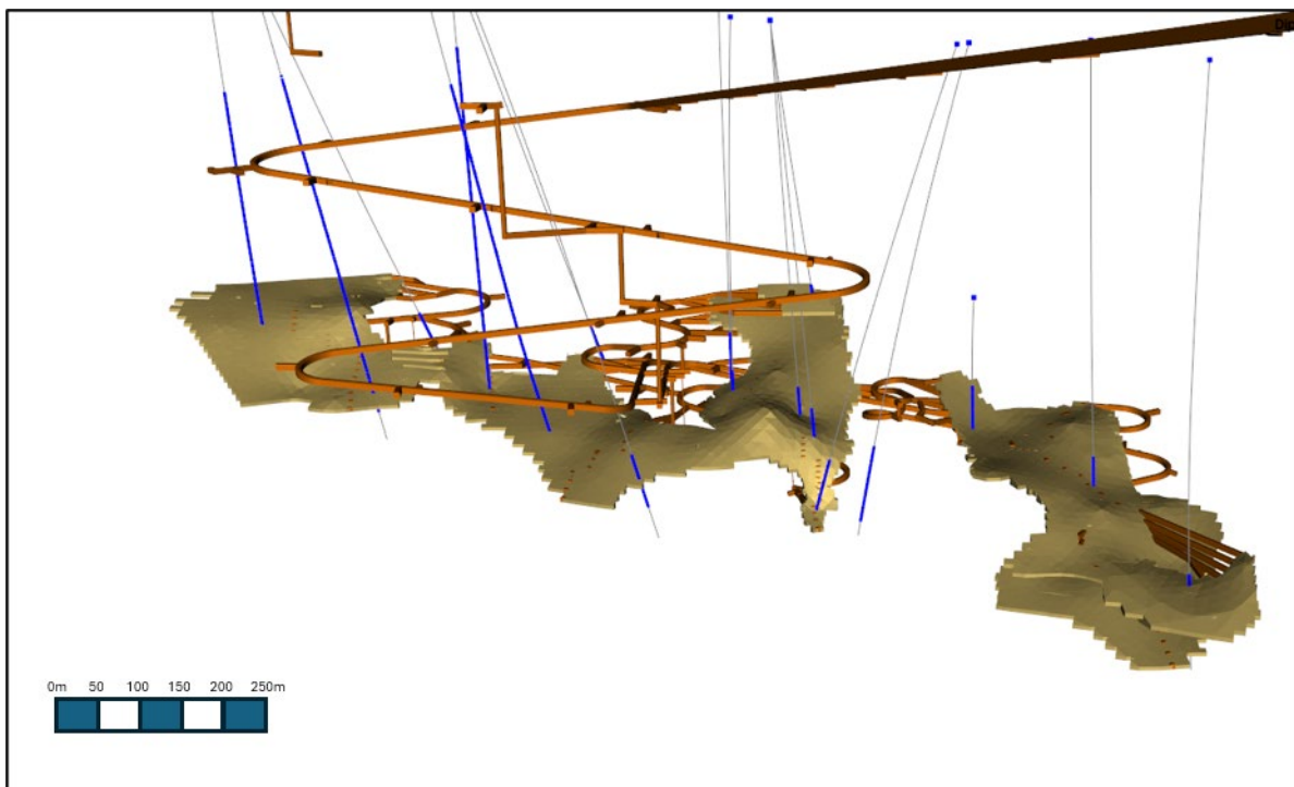
Figure 16.9 5 View looking north of the proposed LCZ at Johnny Lee showing the distribution of geotechnical drilling data collected (Entech, 2025)
