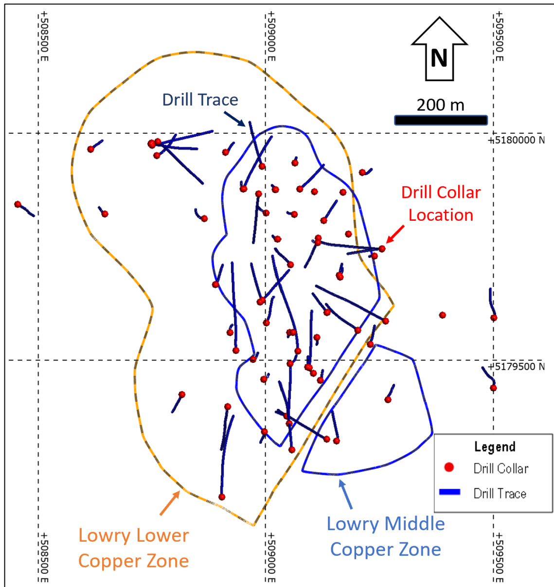
Figure 10.3 Lowry deposit showing drillholes and the surface projection of the Lowry Middle Copper Zone (LMCZ) and Lowry Lower Copper Zone (LLCZ)
