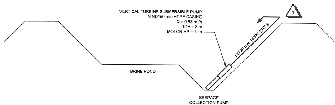
BRINE POND SEEPAGE COLLECTION AND RECYCLE SYSTEM
