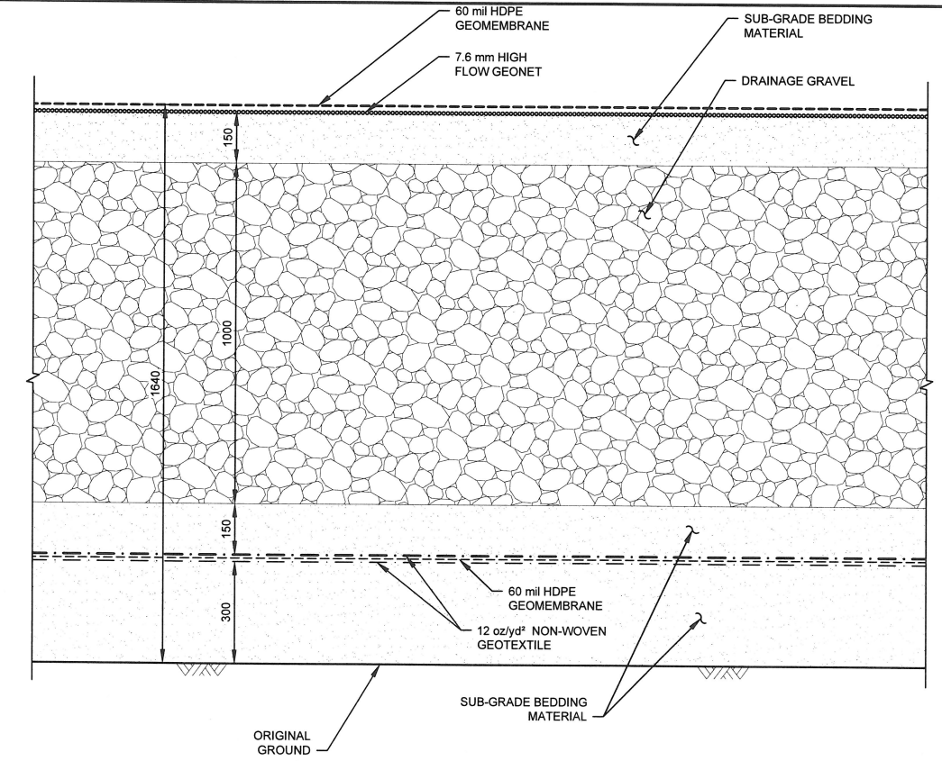
A DETAIL SEEPAGE COLLECTION SUMP LINER DETAIL N.T.S.
