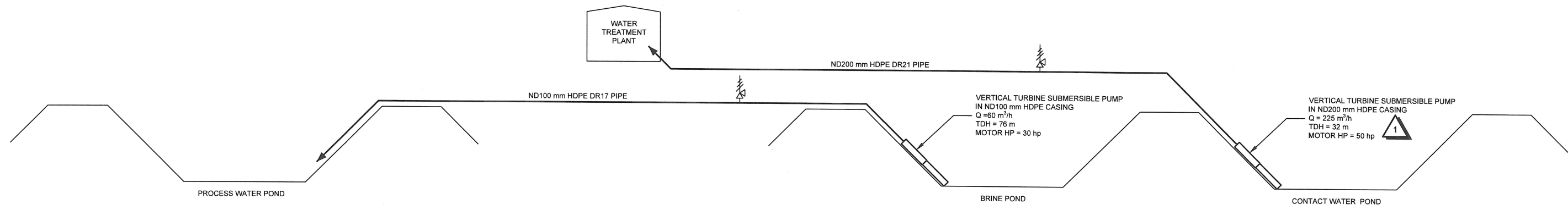
BRINE AND CONTACT WATER RECLAIM SYSTEM
