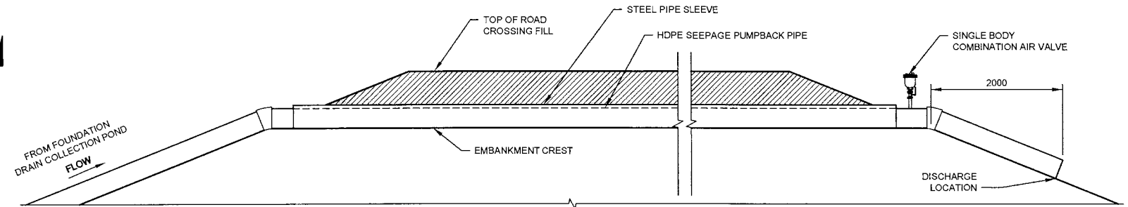
2 2 DETAIL OUTLET AND CREST CROSSING NTS
