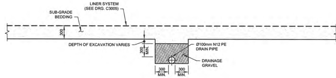
2 C3004 TYPICAL SECTION UPSTREAM EMBANKMENT SLOPE SCALE A
