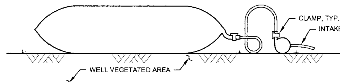
FB FILTER BAG ELEVATION SCALE A
