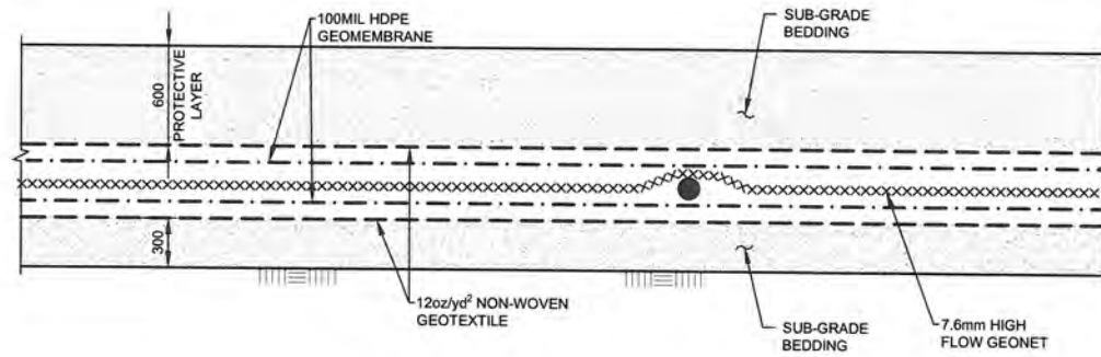
A C2010 DETAIL TYPICAL VIBRATING WIRE PIEZOMETER INSTALLATION IN BASIN DRAIN SCALE A
