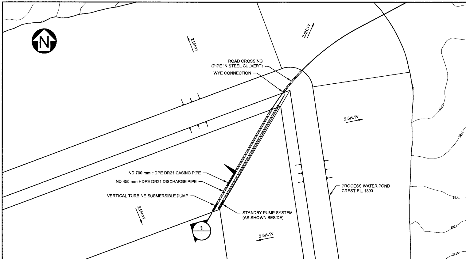
A C6260 DETAIL PROCESS WATER POND INTAKE SCALE A
