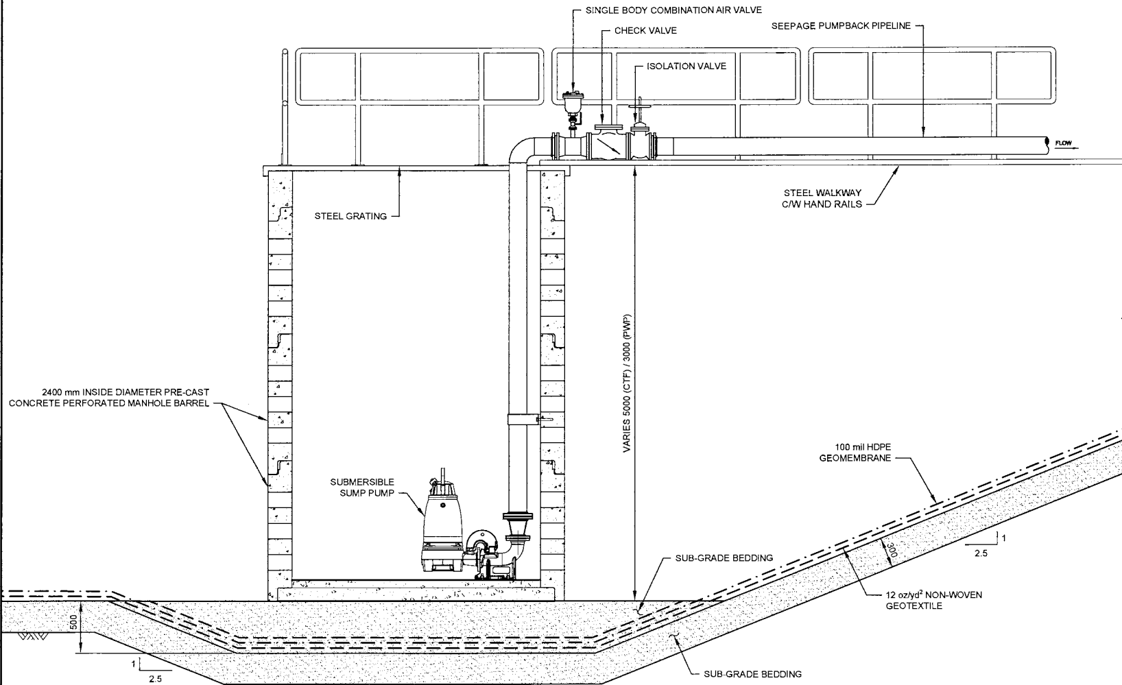
1 SECTION SUMP IN FOUNDATION DRAIN COLLECTION POND NTS
