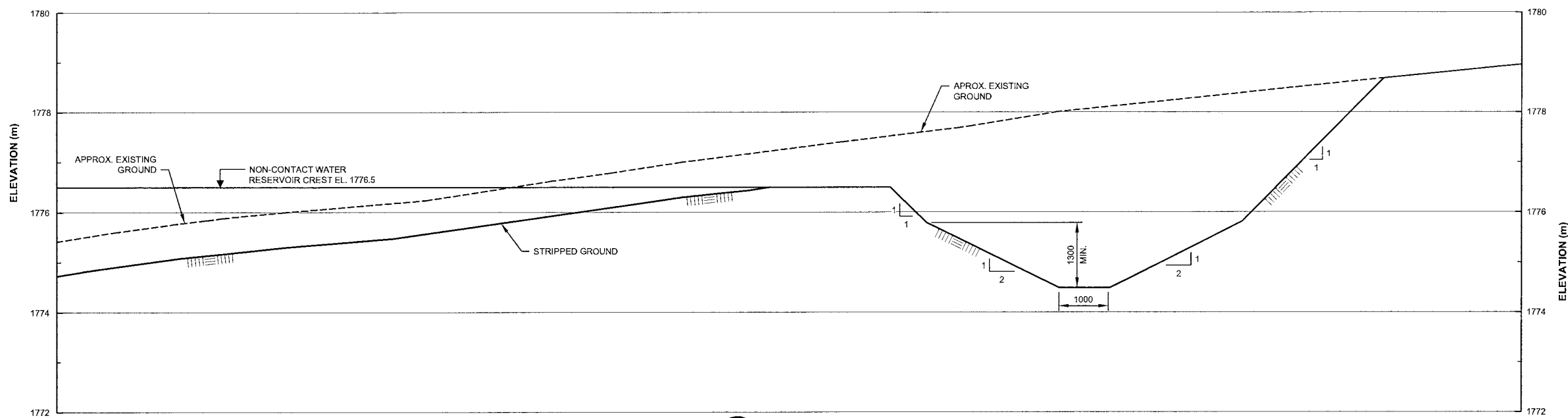
1 SECTION TYPE 1 TYPICAL SPILLWAY SECTION SCALE A
