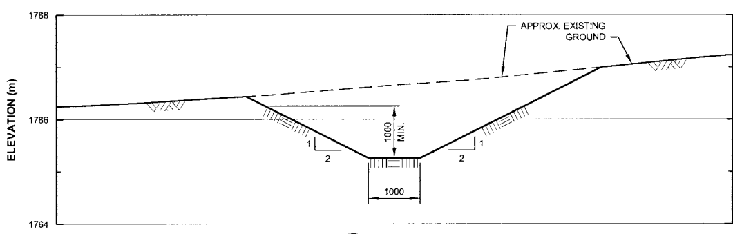
2 SECTION TYPE 2 TYPICAL SPILLWAY SECTION SCALE A
