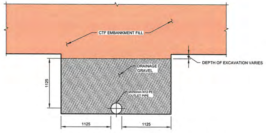
3 C2004 TYPICAL SECTION OUTLET PIPE (BELOW EMBANKMENT FILL) SCALE A
