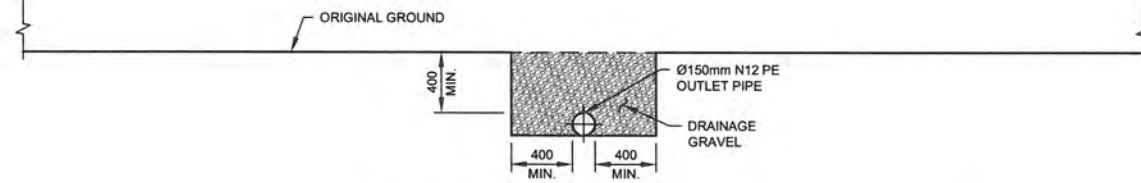
4 C3004 TYPICAL SECTION OUTLET PIPE (NO OVERLYING EMBANKMENT FILL) SCALE A
