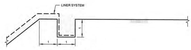
B DETAIL ANCHOR TRENCH DETAIL SCALE C
