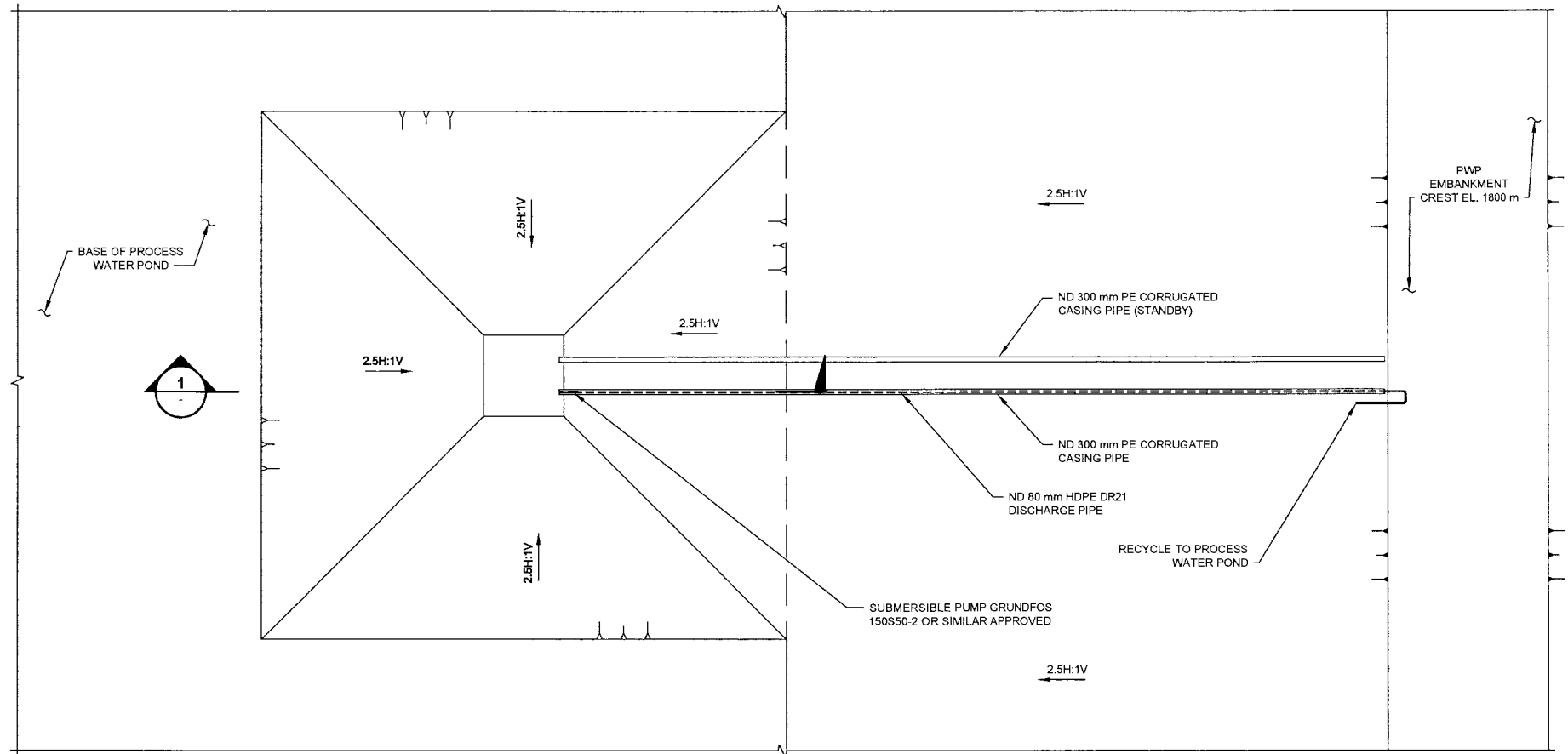
A DETAIL C6510 PWP SEEPAGE COLLECTION SUMP SCALE A
