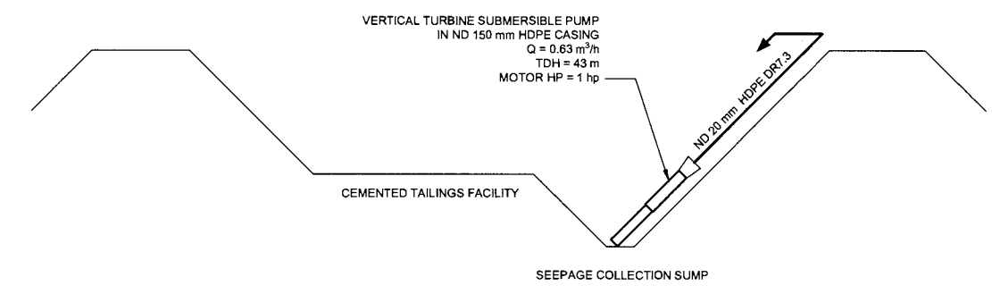
CTF SEEPAGE COLLECTION AND RECYCLE SYSTEM
