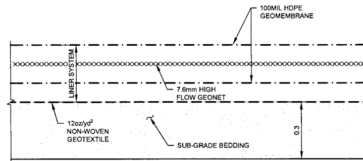
C DETAIL LINER SYSTEM DETAILS
