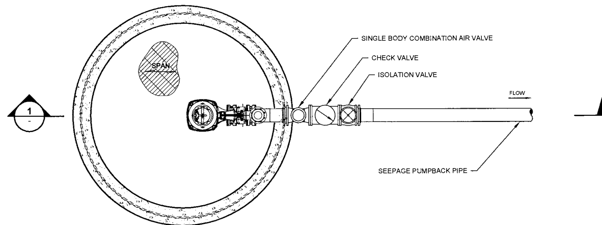
1 DETAIL SUMP IN FOUNDATION DRAIN COLLECTION POND NTS
