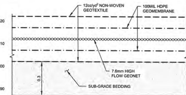
C DETAIL LINER SYSTEM DETAILS SCALE D
