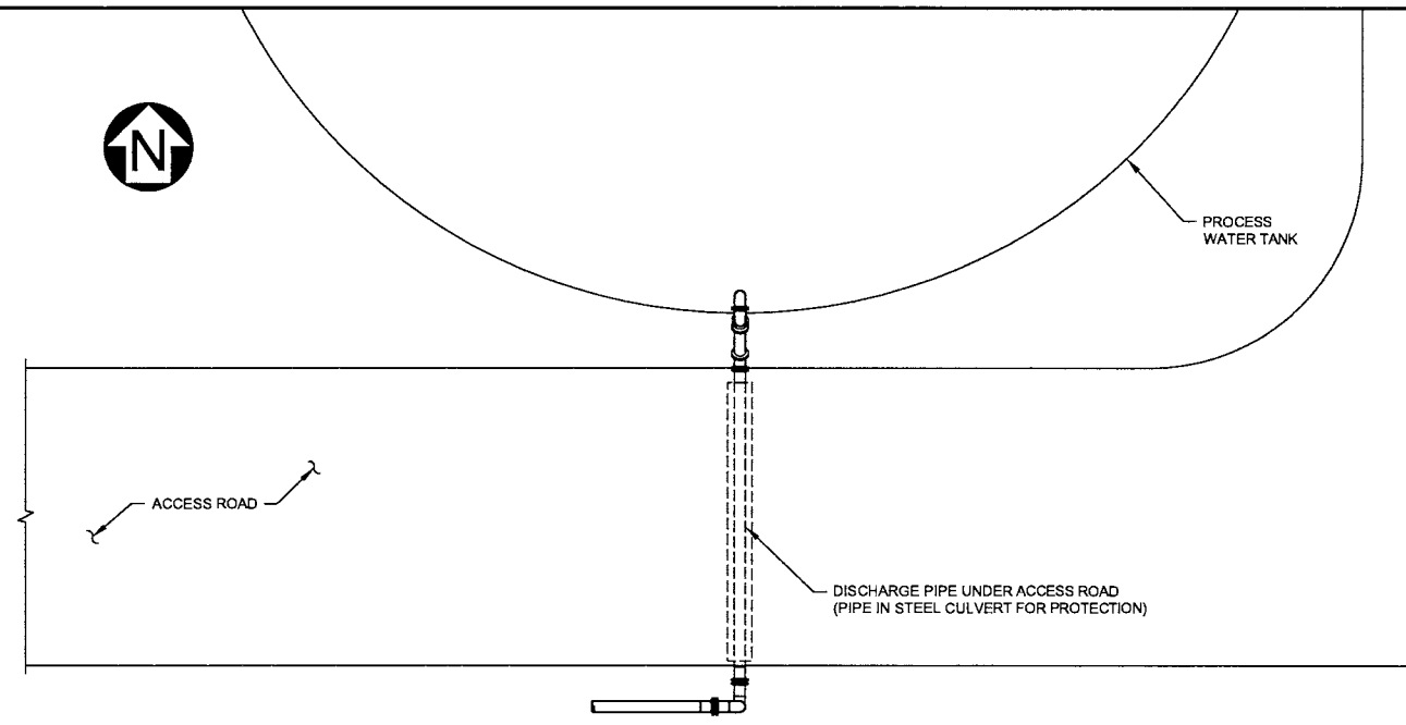
B C6260 DETAIL DISCHARGE TO PROCESS WATER TANK SCALE B
