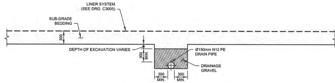
1 C3004 TYPICAL SECTION BASIN FLOOR (BELOW LINER) SCALE A
