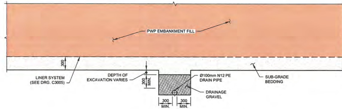
3 C3004 TYPICAL SECTION BELOW EMBANKMENT FILL SCALE A
