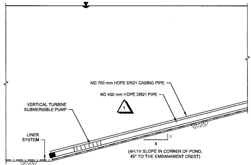
1 C6260 SECTION PROCESS WATER POND INTAKE SCALE B
